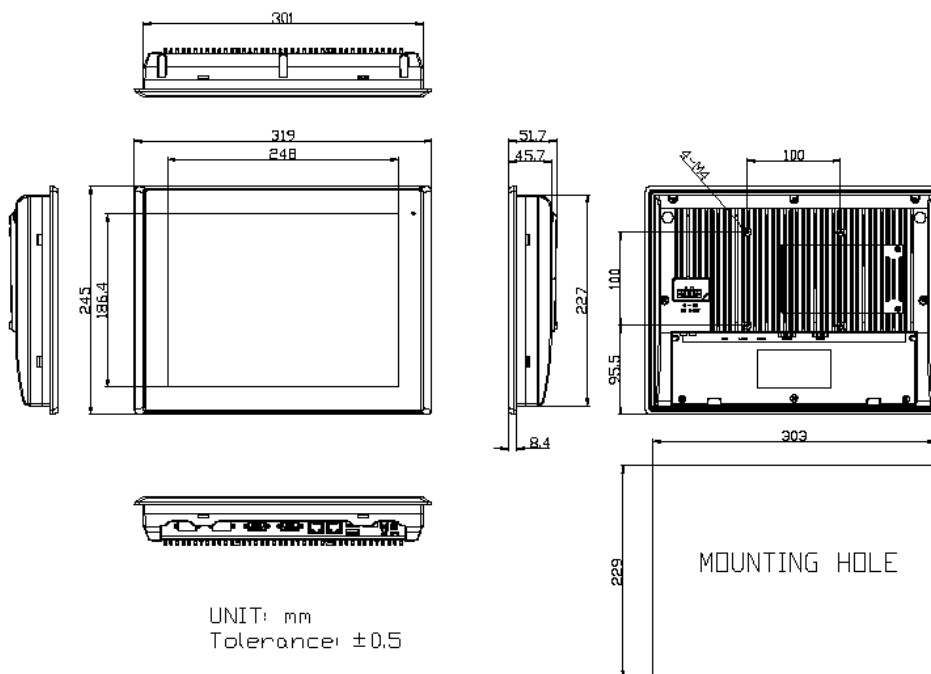
Figure 1.4: Dimensions of ARCHMI-812AP/AR/AG(H)
