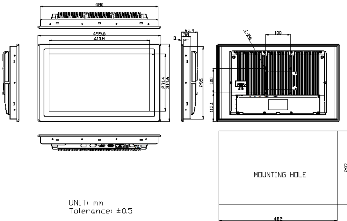
Figure 1.8: Dimensions of ARCHMI-818AP/AR/AG(H)
