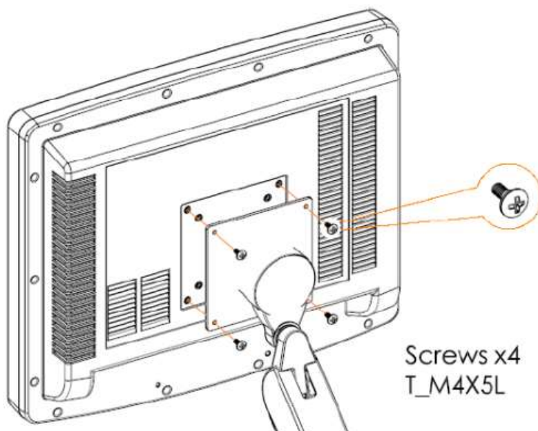
Figure 1.31: ARCHMI-8XXX Series VESA Mounting
