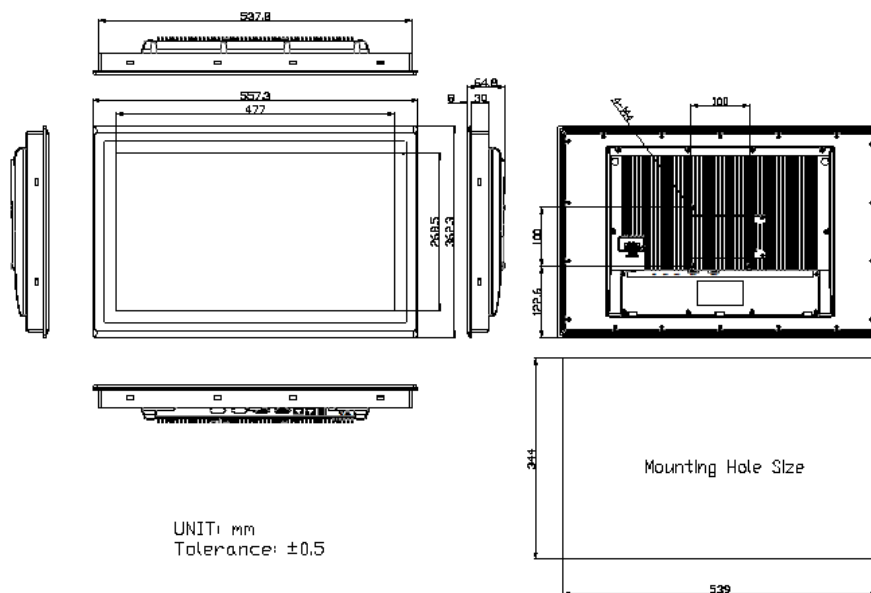
Figure 1.10: Dimensions of ARCHMI-821AP/AR/AG(H)
