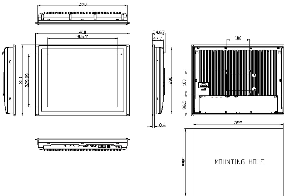
Figure 1.5: Dimensions of ARCHMI-815AP/AR/AG(H)
