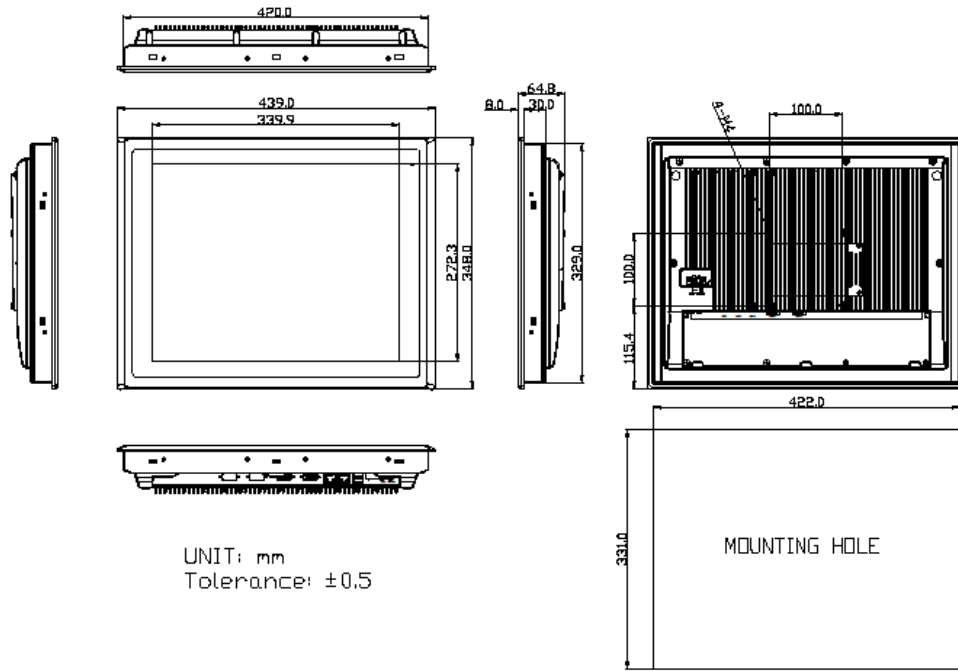
Figure 1.7: Dimensions of ARCHMI-817AP/AR/AG (H)
