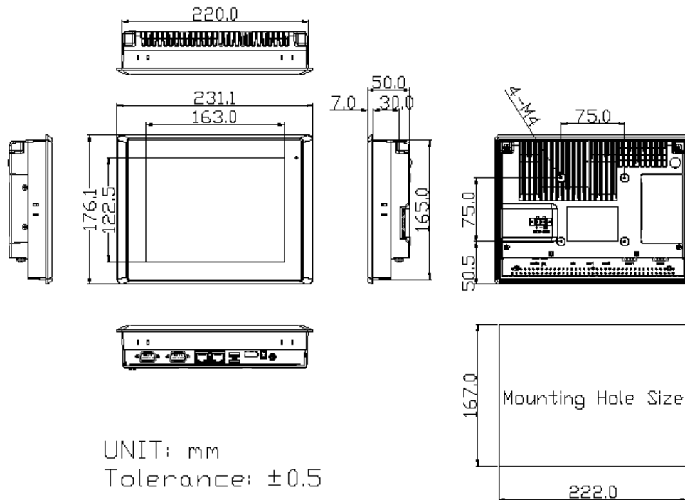
Figure 1.2: Dimensions of ARCHMI-808AP/AR/AG(H)
