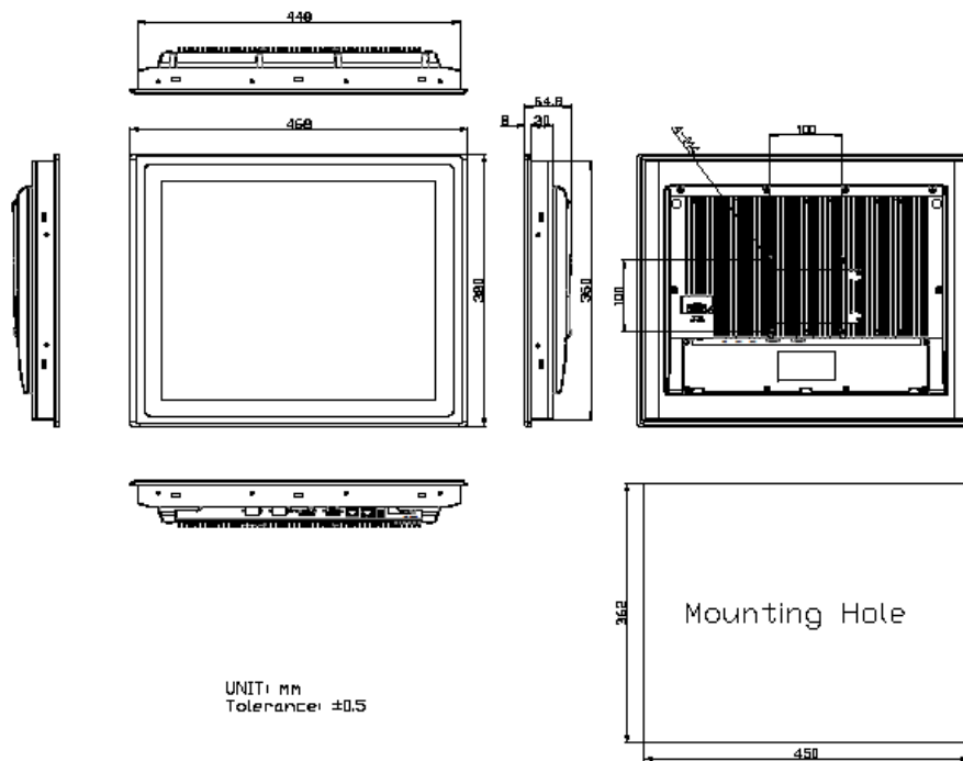
Figure 1.9: Dimensions of ARCHMI-819AP/AR/AG(H)
