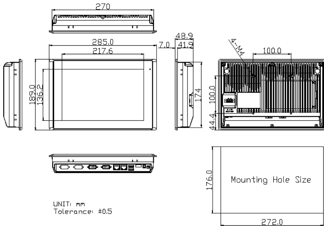
Figure 1.3: Dimensions of ARCHMI-810AP/AR/AG(H)
