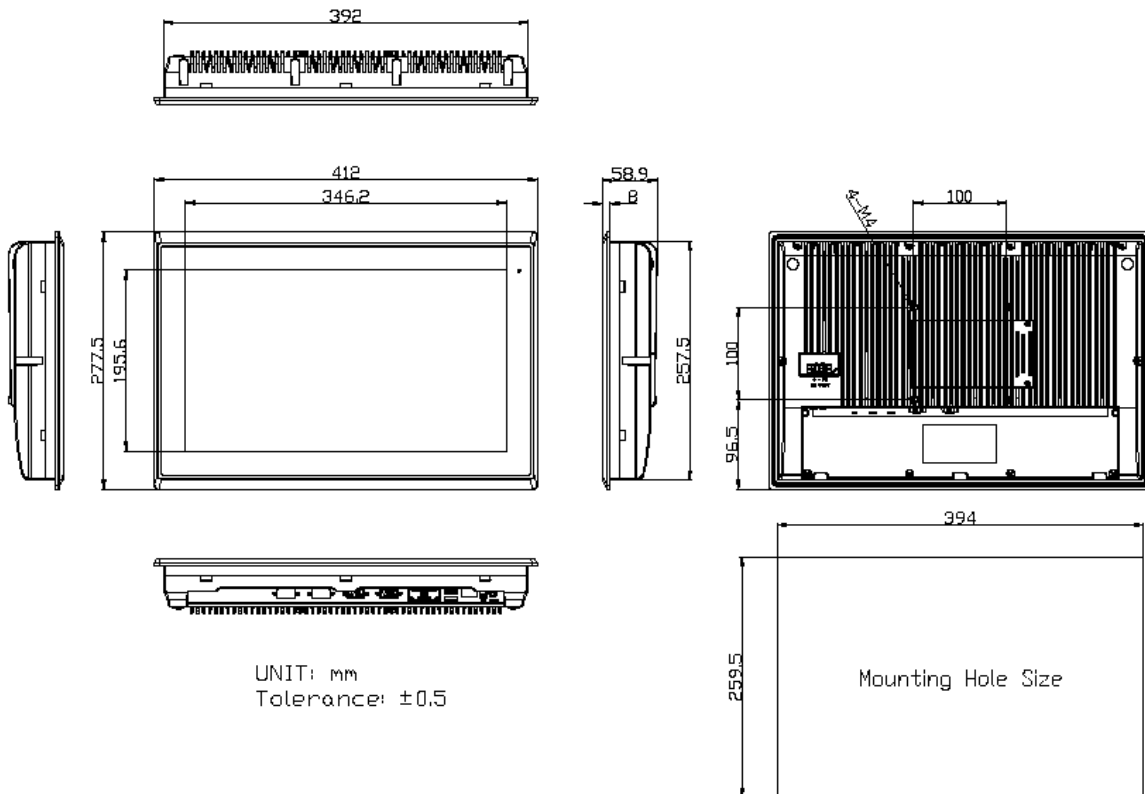
Figure 1.6: Dimensions of ARCHMI-816AP/AR/AG(H)
