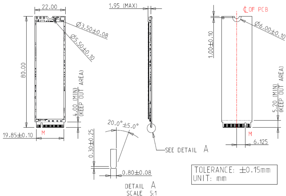
Figure 2: Innodisk M.2 (P80) 3TE6 with heat-spreading copper layer diagram
