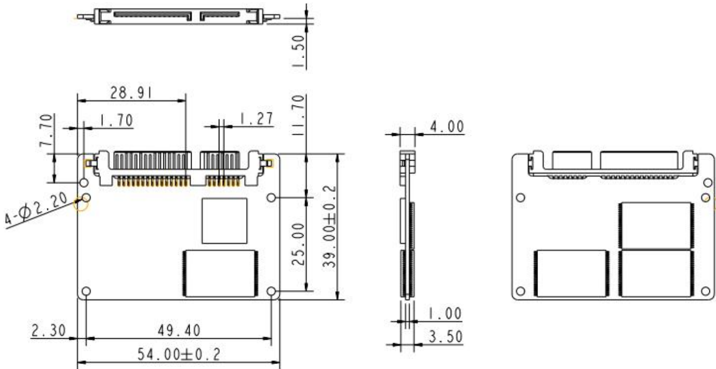
Figure 4: SATA Slim D150Q mechanical dimensions (*Tolerance is ±0.2mm)
