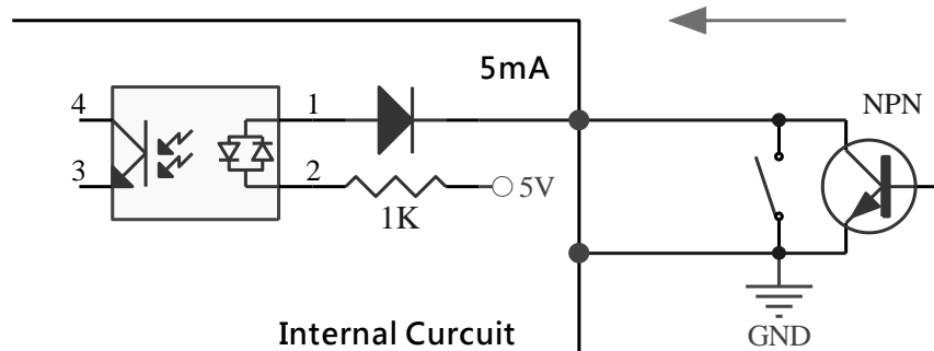
Figure of ALM wiring for NPN sink mode
