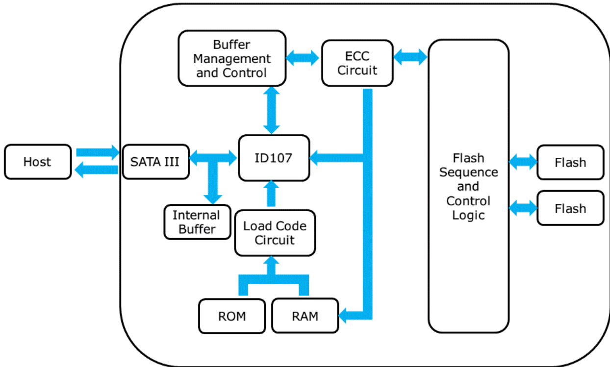
Figure 2: Innodisk SATADOM-SH TPYE D 3SE Block Diagram
