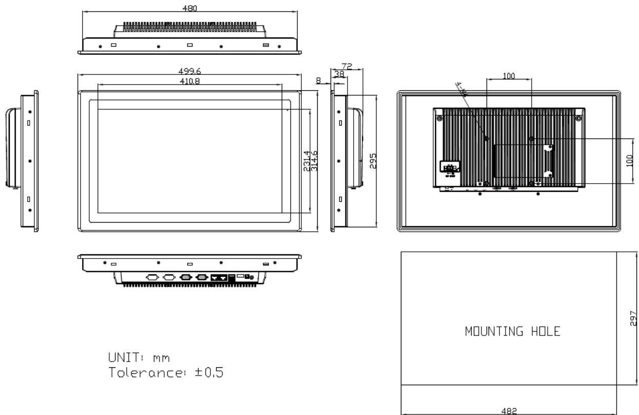
Figure 1.5: Dimensions of ARCHMI-918(P)
