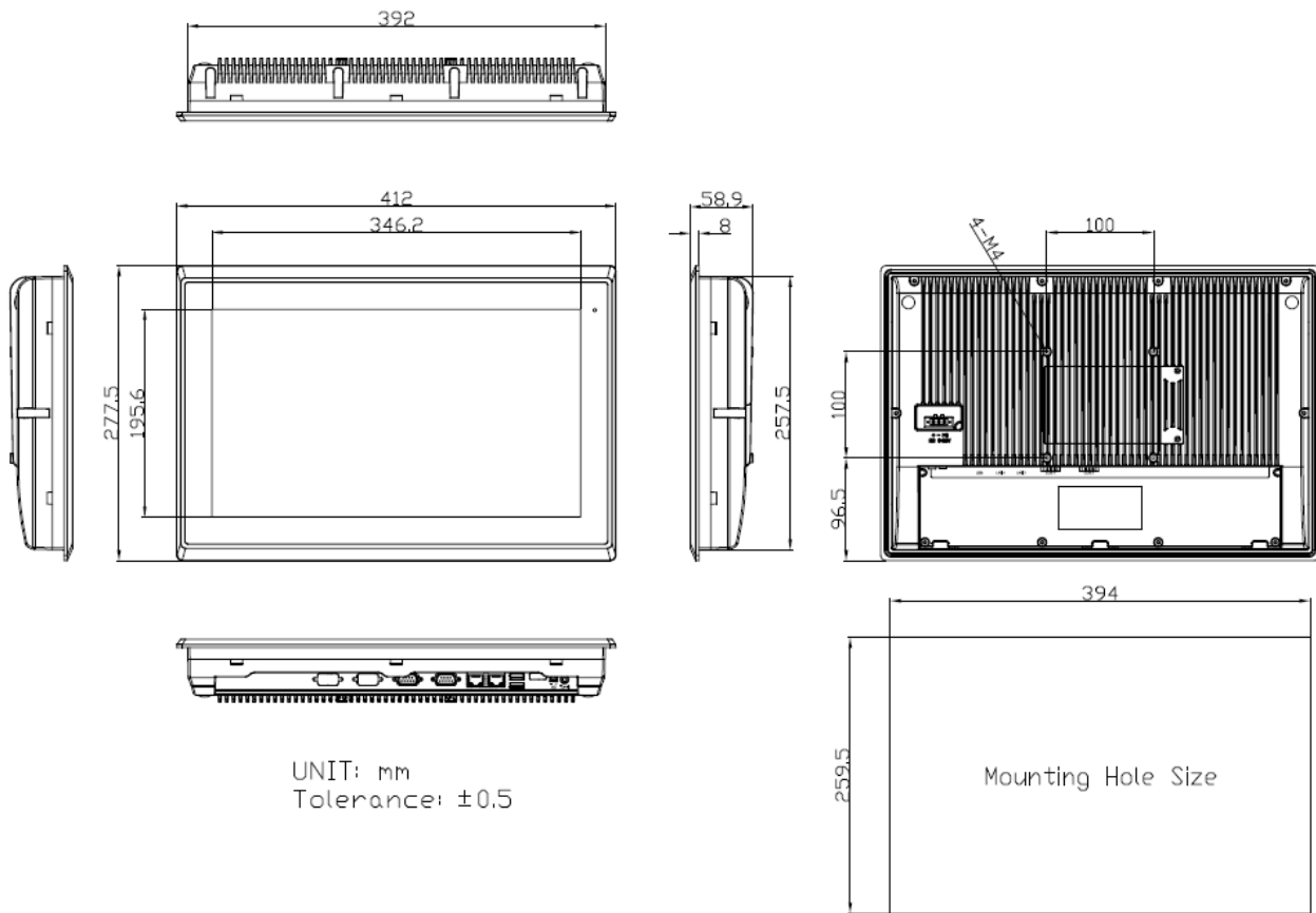
Figure 1.3: Dimensions of ARCHMI-916(P)
