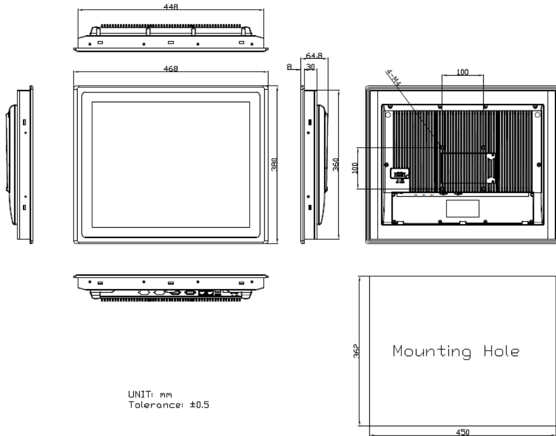
Figure 1.6: Dimensions of ARCHMI-919(P)
