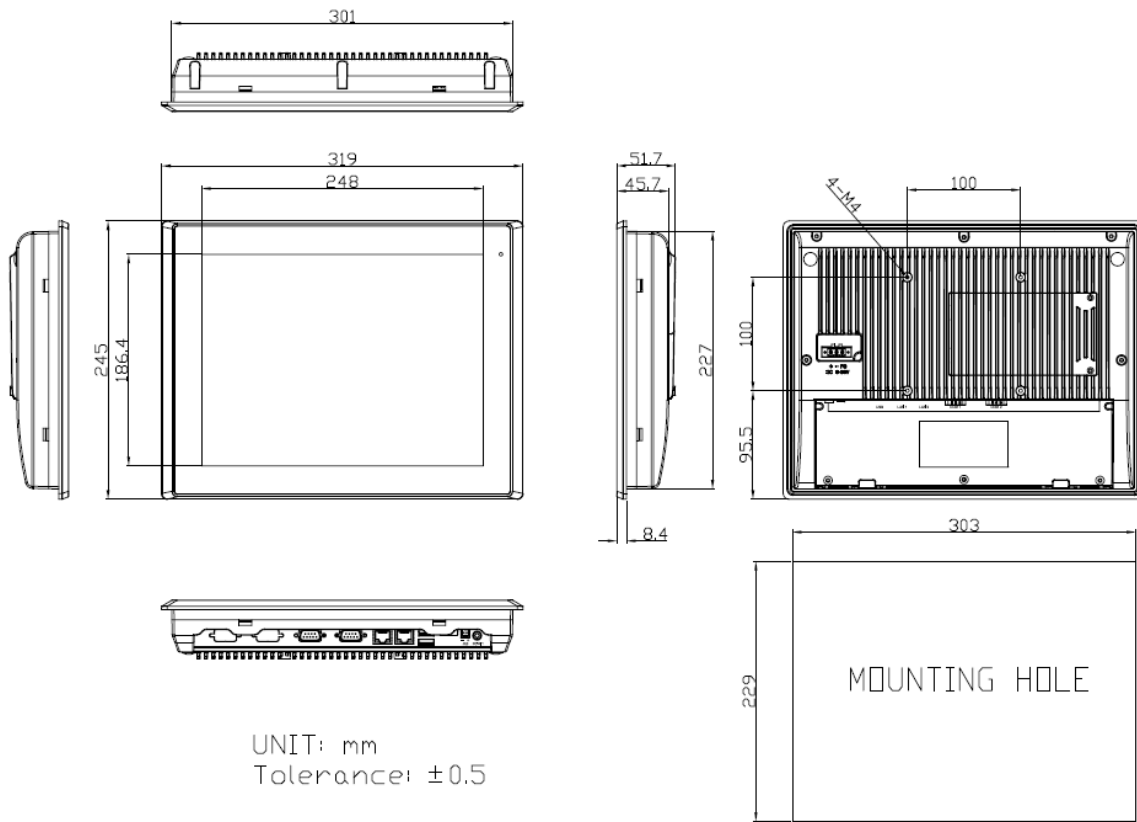
Figure 1.1: Dimensions of ARCHMI-912(P)
