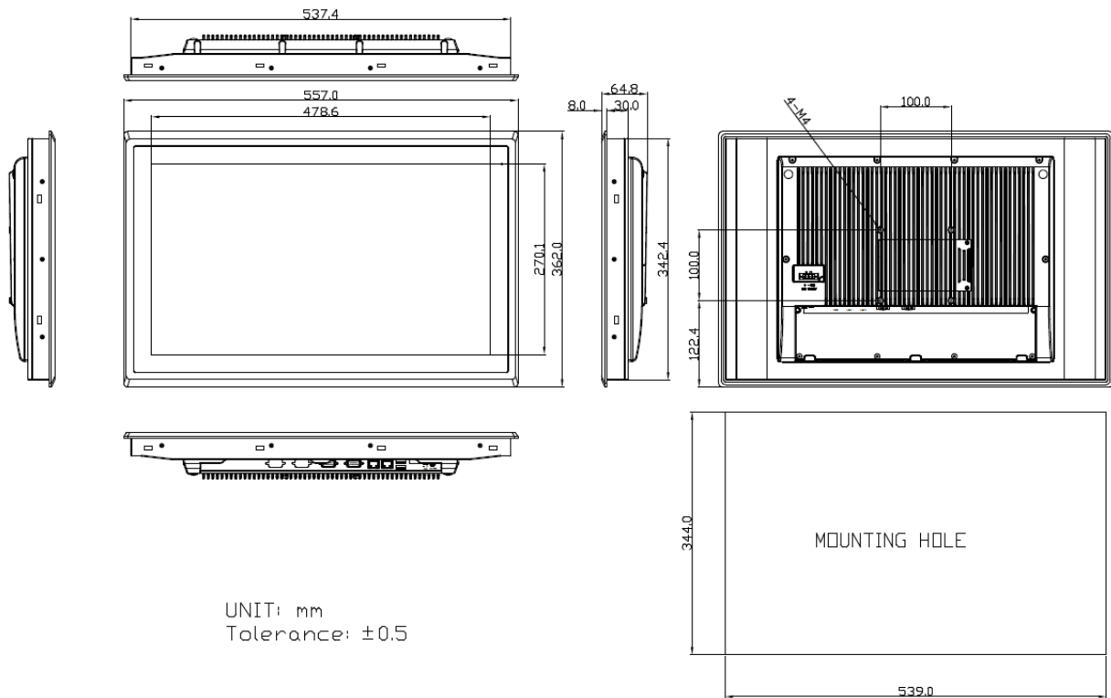
Figure 1.7: Dimensions of ARCHMI-921(P)
