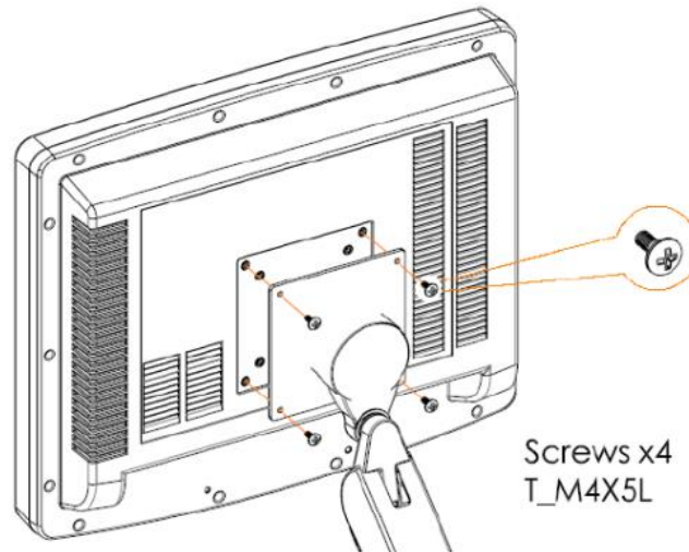
Figure 1.16: ARCHMI Series VESA Mounting
