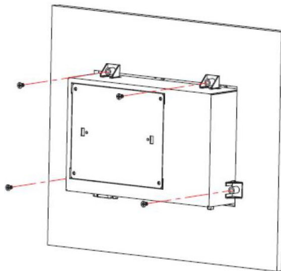
Figure 1.17: ARCHMI Series Panel Mounting
