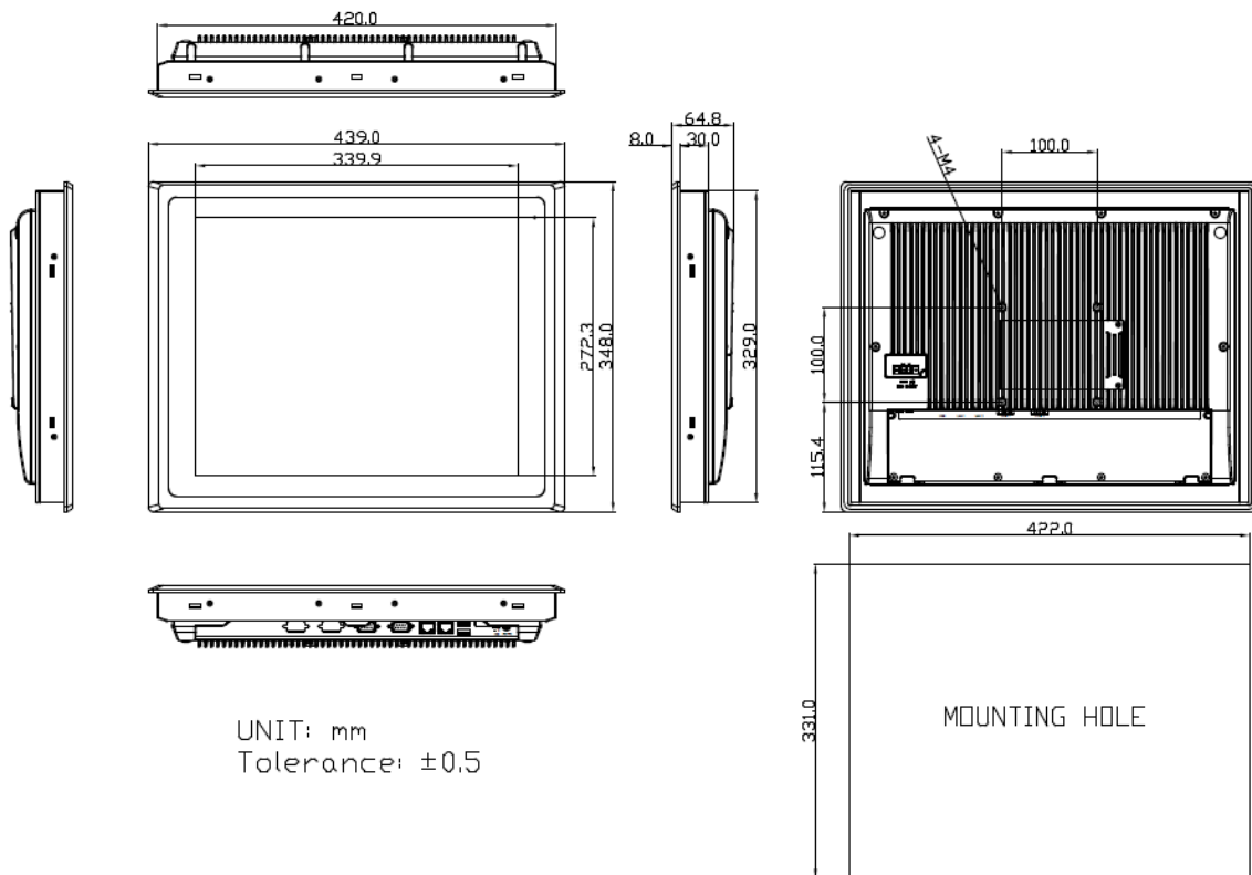
Figure 1.4: Dimensions of ARCHMI-917(P)
