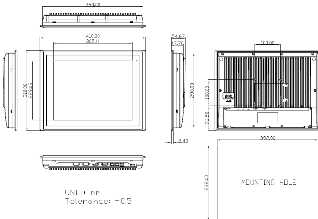
Figure 1.2: Dimensions of ARCHMI-915(P)
