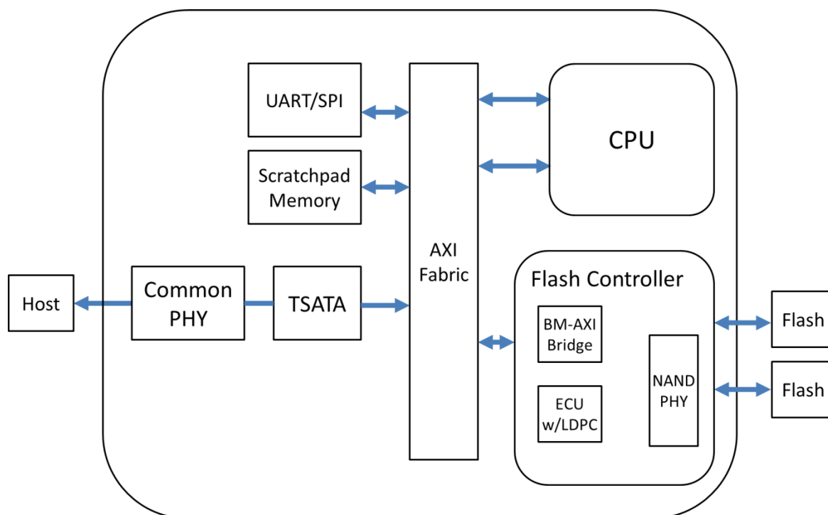
Figure 3: Innodisk SATADOM-SH 3SE4 Block Diagram
