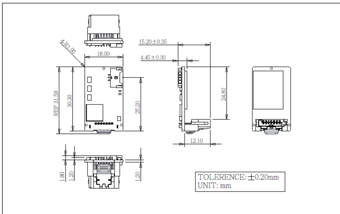
Figure 2: Innodisk SATADOM-SH 3SE4 mechanical diagram
