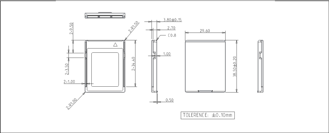
Figure 2: Innodisk CFexpress 3ME2 diagram
