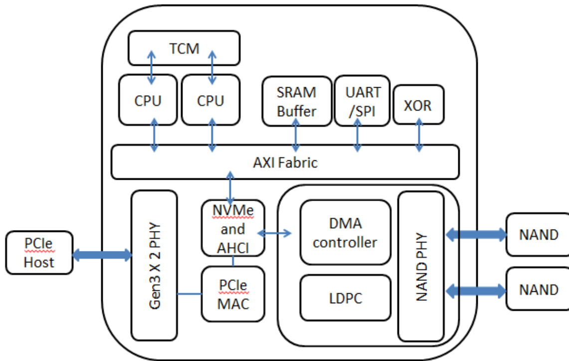
Figure 3: Innodisk CFexpress 3ME2 Block Diagram
