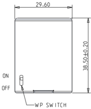
Figure 5: Write Protect Switch
