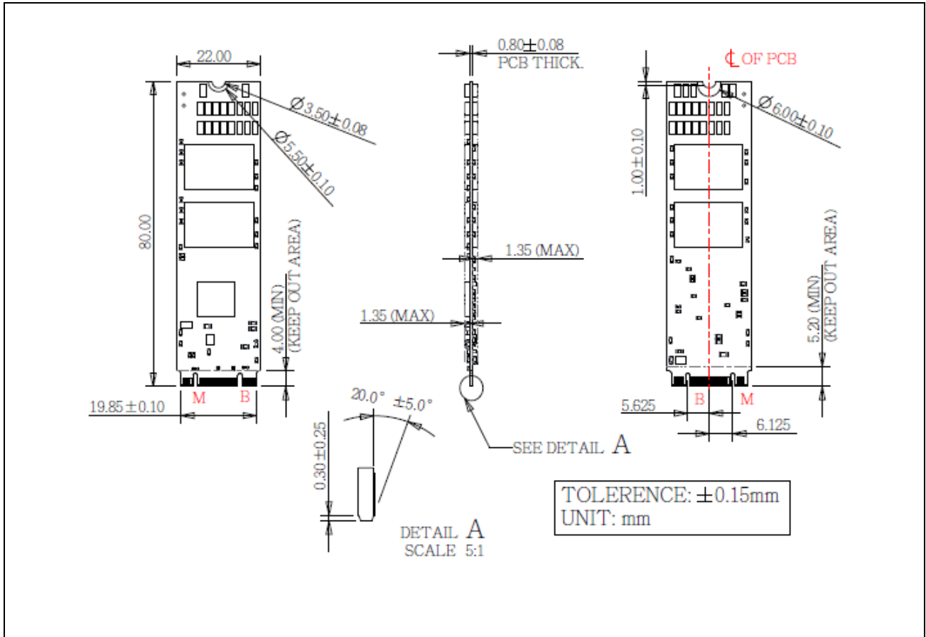
Figure 2: Innodisk M.2 (P80) 3IE2 diagram
