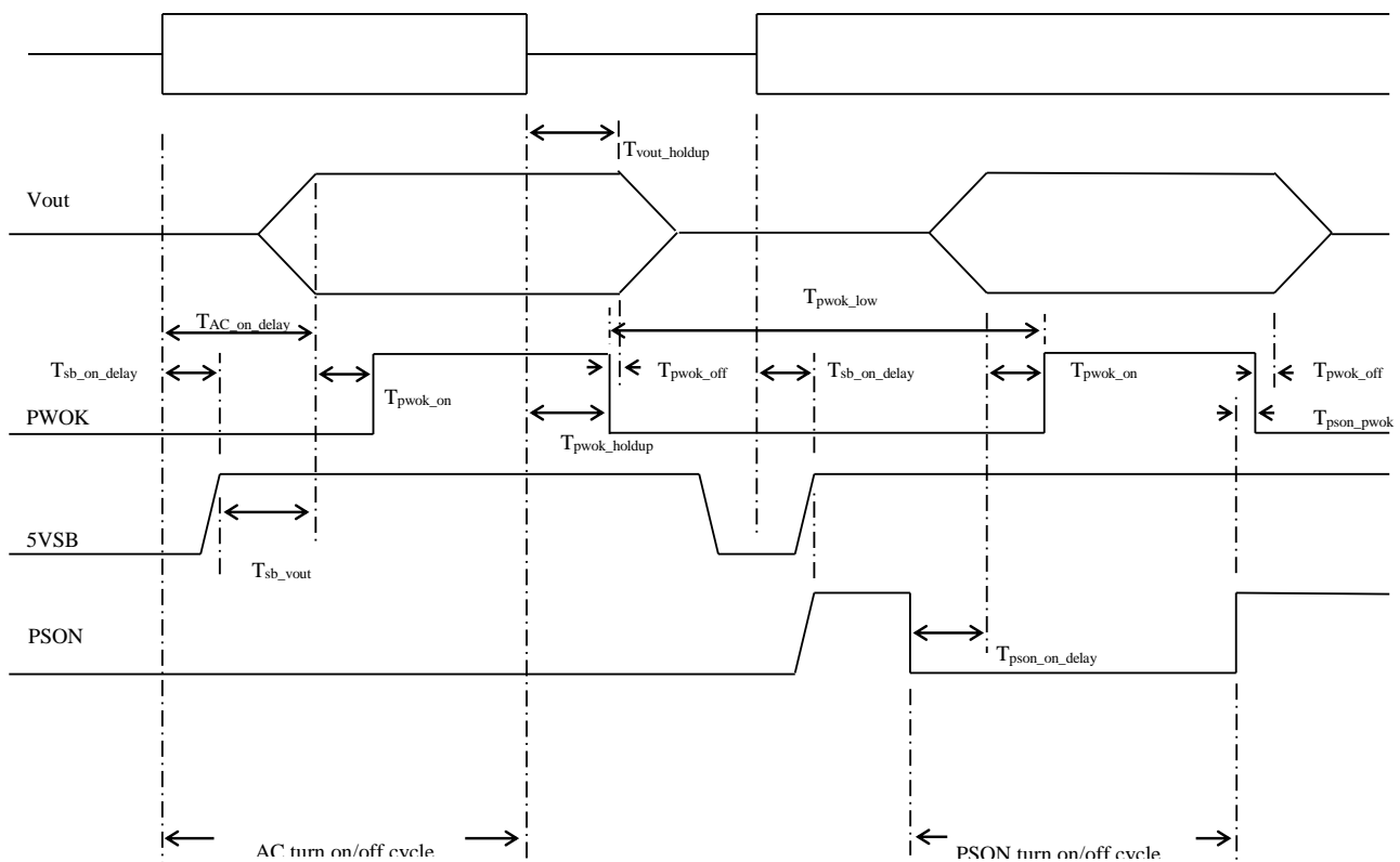
Figure 2: Timing Diagram
