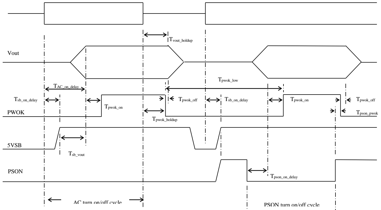
Figure 3 Timing Diagram
