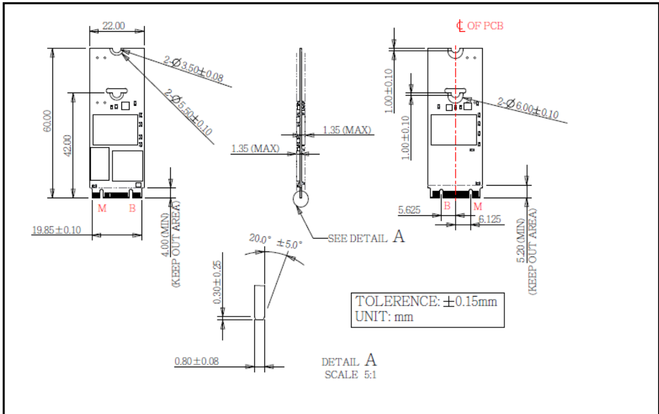
Figure 2: Innodisk M.2 (S60) 3MG2-P Diagram
