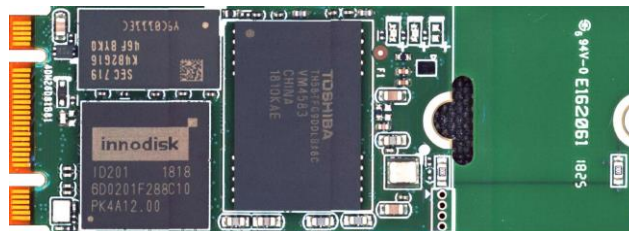
Figure 1: Innodisk M.2 (S60) 3MG2-P
