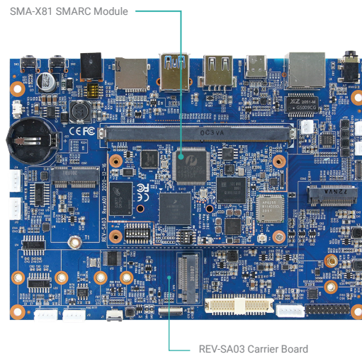
▲ SMA-X81 SMARC Module installed on REV-SA03 Carrier Board
