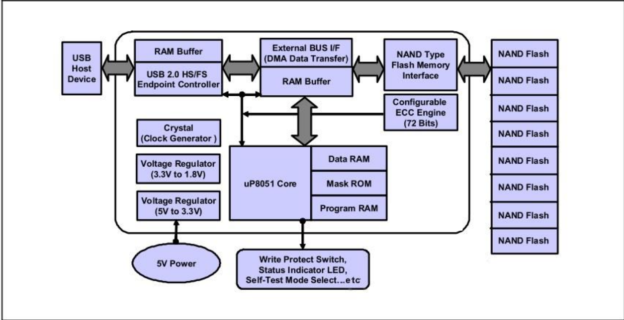
Figure 2: USB Drive 2ME2 Block Diagram
