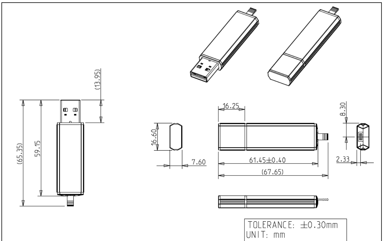
Figure 4: USB Drive 2ME2 mechanical dimensions (with write-protection function)
