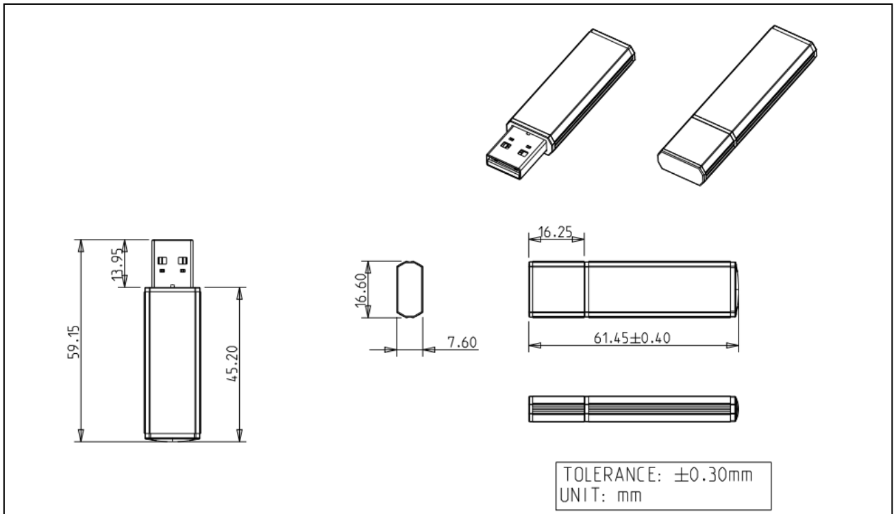
Figure 3: USB Drive 2ME2 mechanical dimensions
