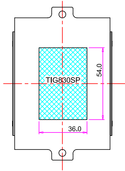
Bottom Surface Thermal Grease Pre-Print Zone Scale 3/4 : 1
