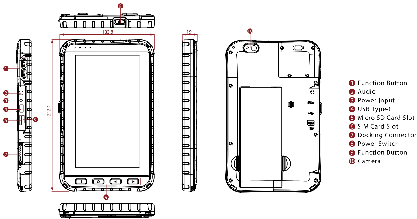
M700DQ8-7inch sunlight readable android tablet
