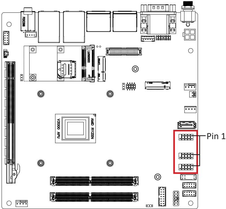
USB 2.0 header
