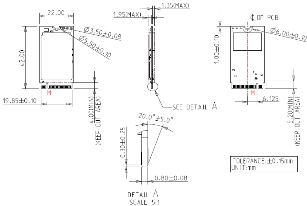
Figure 3: Innodisk M.2 (P42) 3TE6 with heat-spreading copper layer diagram
