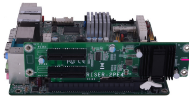
RISER-2PE4 Connected to the Motherboard
