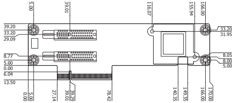
Mechanical Drawing
