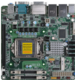
Motherboard (SB102-D)
