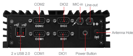
Rear I/O
