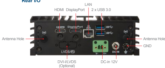
Rear I/O
