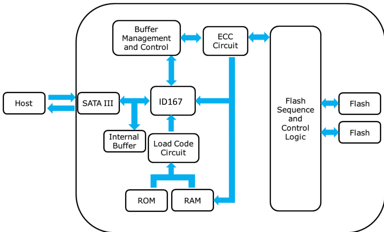
Figure 2: Innodisk SATADOM-ML 3MG-P Block Diagram
