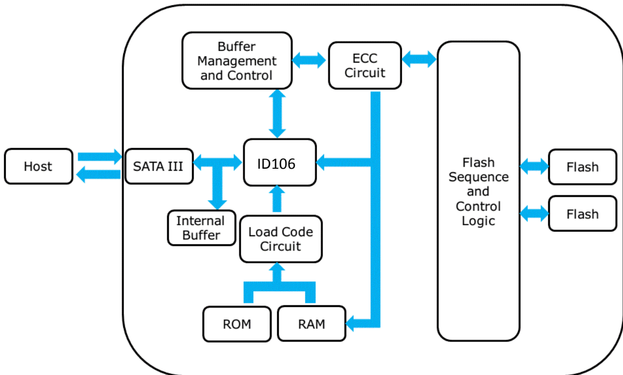
Figure 2: Innodisk SATADOM-ML 3SE Block Diagram
