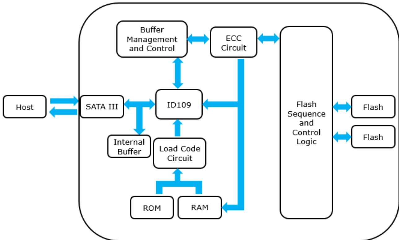
Figure 3: Innodisk SATADOM-SH type C 3SE3 Block Diagram
