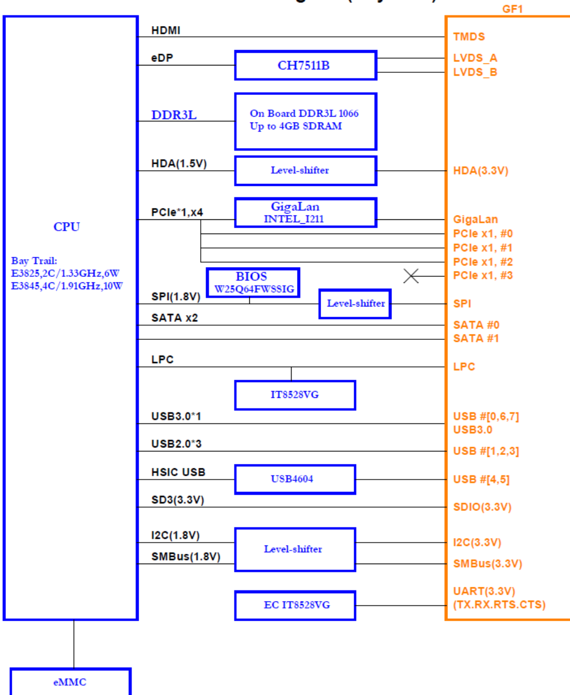
EQM-BYT2 Block diagram (Bay Trail)
