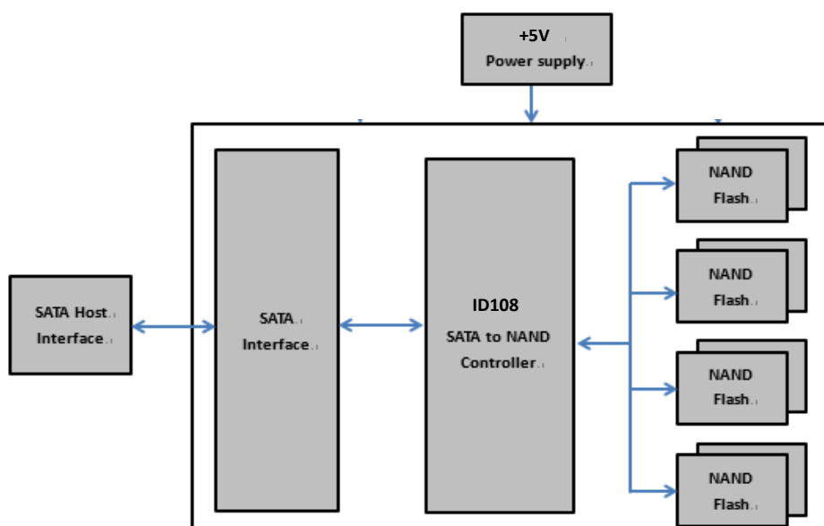
Figure 2: Innodisk ServerDOM-V 3IE3 Block Diagram
