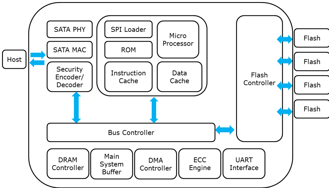
Figure 2: Innodisk 2.5" SATA SSD 3IE6-P Block Diagram
