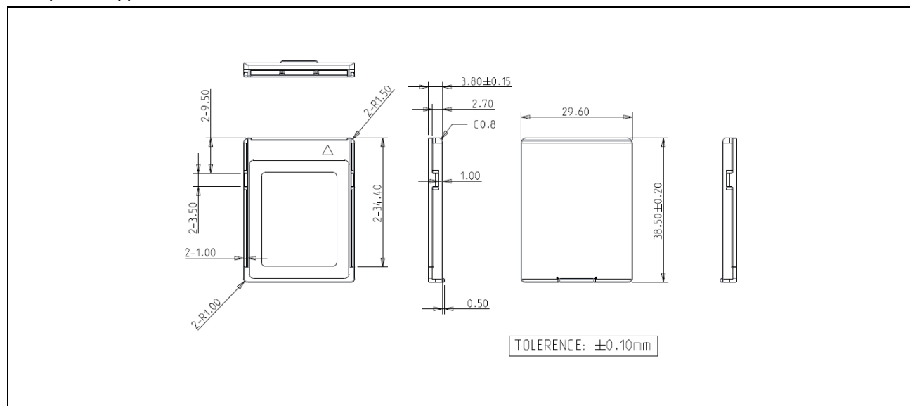
Figure 2: Innodisk CFexpress 4TE3 diagram
