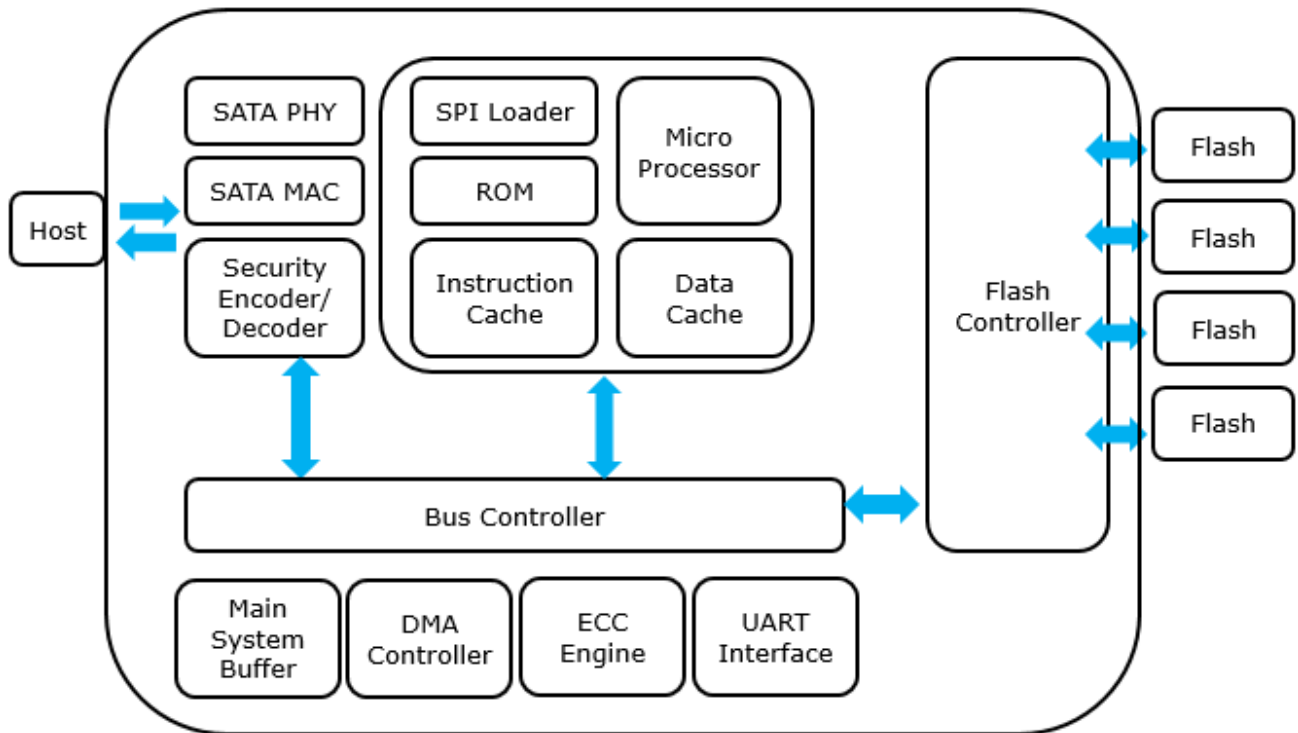
Figure 2: Innodisk M.2 (S42) 3ME2 Block Diagram
