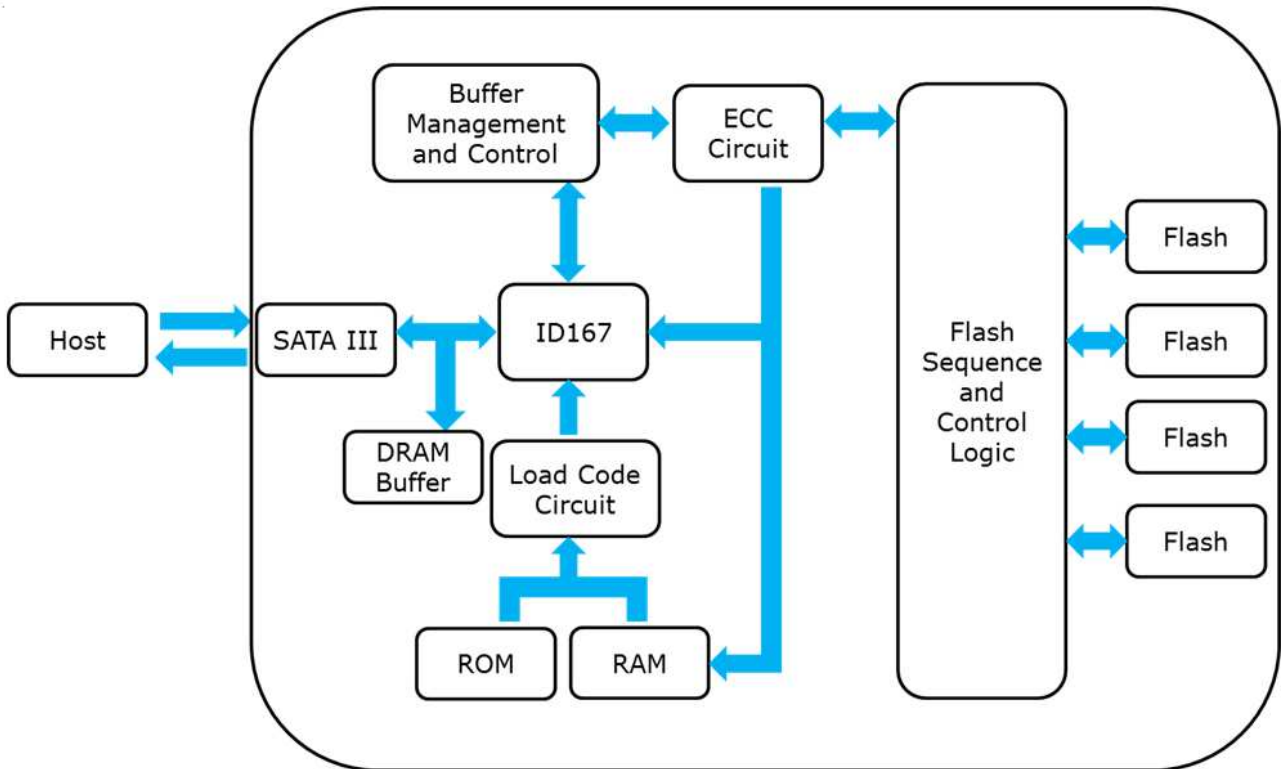
Figure 2: Innodisk FiD 1.8" SATA SSD 3SR-P Block Diagram
