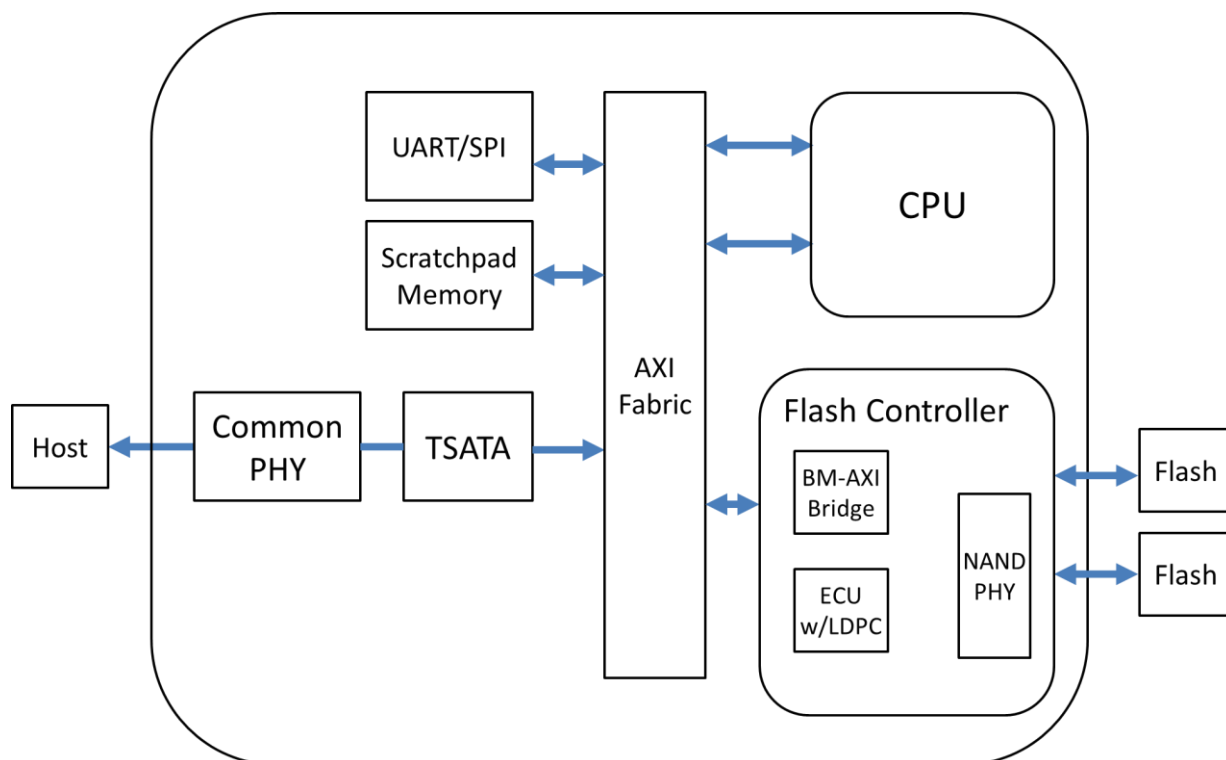
Figure 3: Innodisk SATADOM-SH 3ME4 Block Diagram
