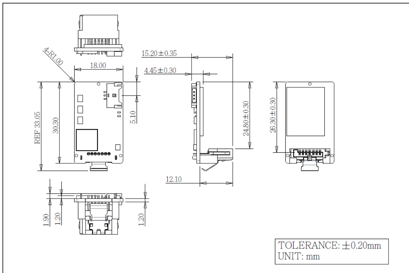
Figure 2: Innodisk SATADOM-SH 3ME4 mechanical diagram
