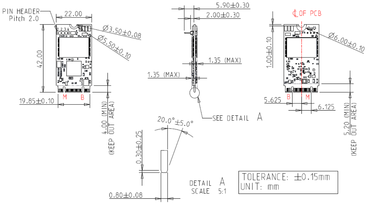
Figure 3: Innodisk M.2 (S42) 3T07 diagram (TSOP) with Vertical Pin Headers
