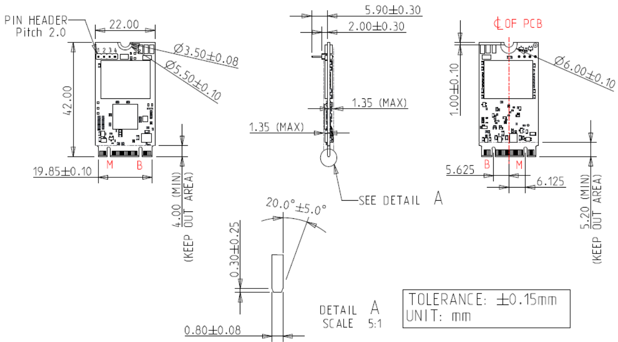
Figure 5: Innodisk M.2 (S42) 3T07 diagram (BGA for 512GB model) with Vertical Pin Headers
