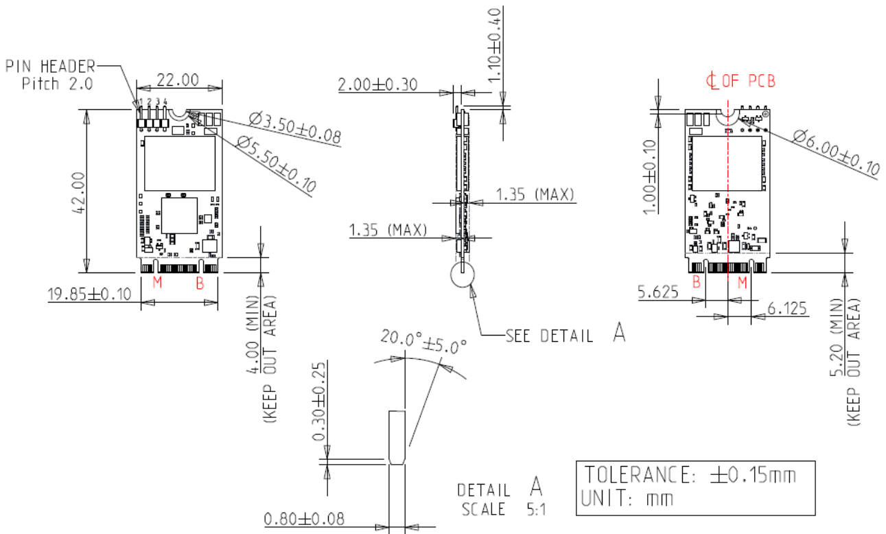
Figure 3: Innodisk M.2 (S42) 3T07 diagram (TSOP) with Vertical Pin Headers
