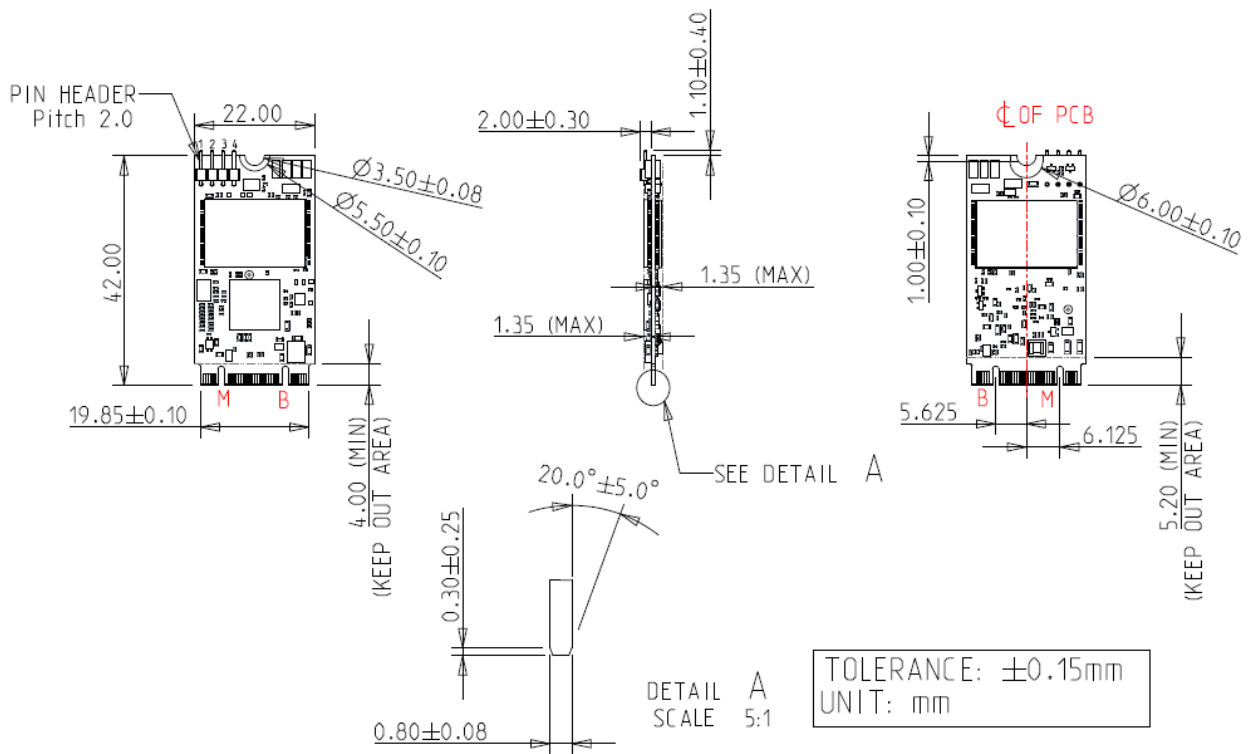
Figure 2: Innodisk M.2 (S42) 3T07 diagram (TSOP) with Horizontal Pin Headers
