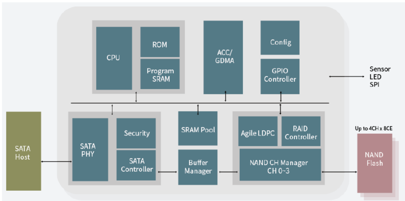
Figure 6: Innodisk M.2 (S42) 3TO7 Block Diagram
