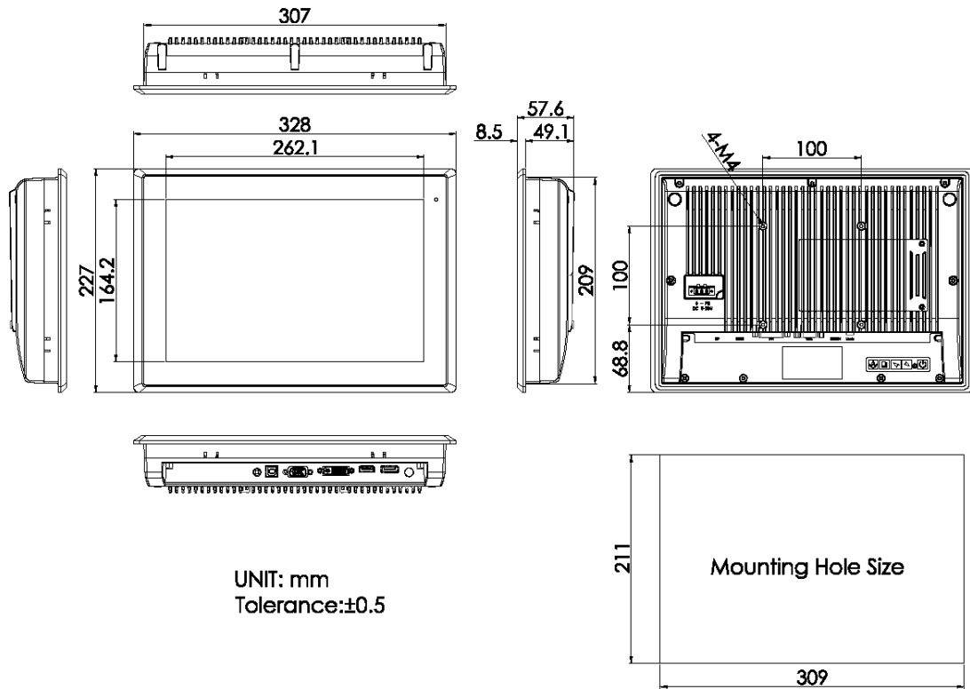
Figure 1.5: Dimensions of ARCDIS-112WAPRG(H)
