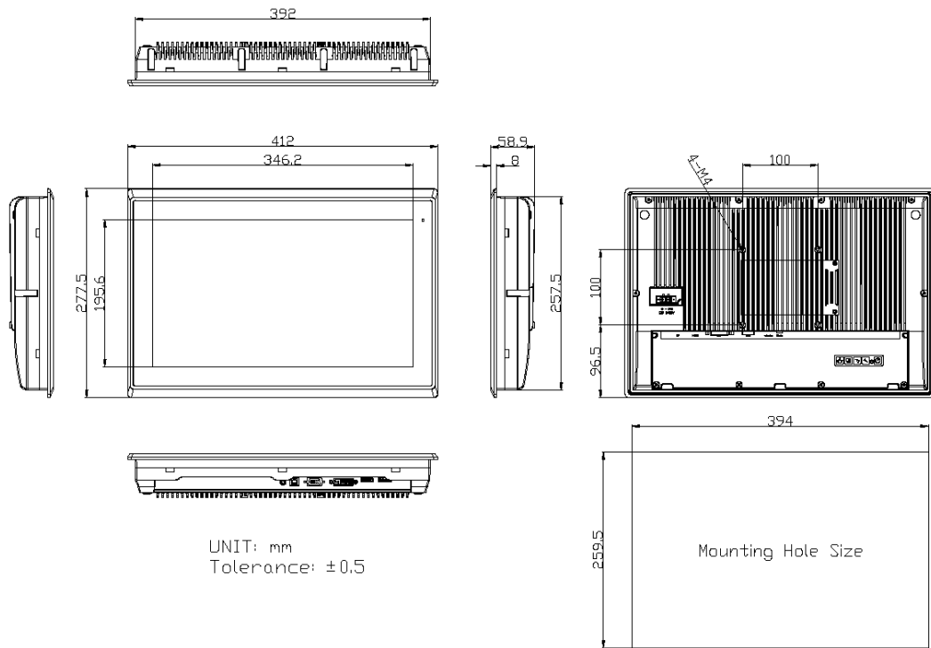
Figure 1.7: Dimensions of ARCDIS-116APRG(H)
