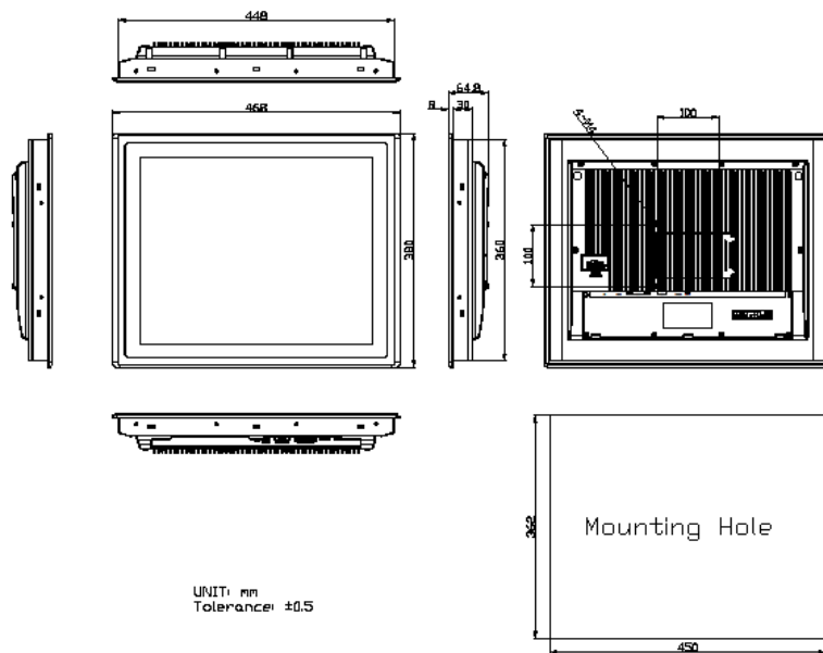
Figure 1.10: Dimensions of ARCDIS-119APRG(H)
