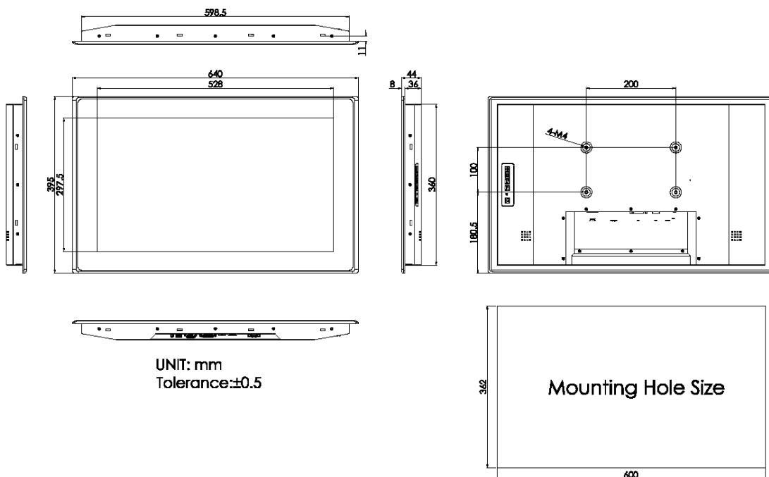
Figure 1.12: Dimensions of ARCDIS-124APG(H)
