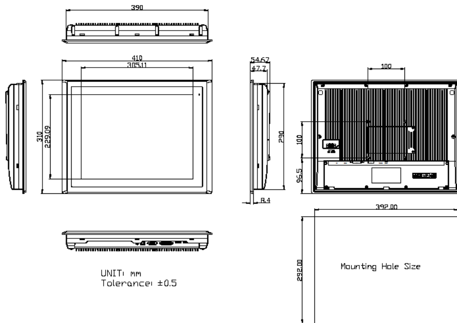
Figure 1.6: Dimensions of ARCDIS-115APRG(H)
