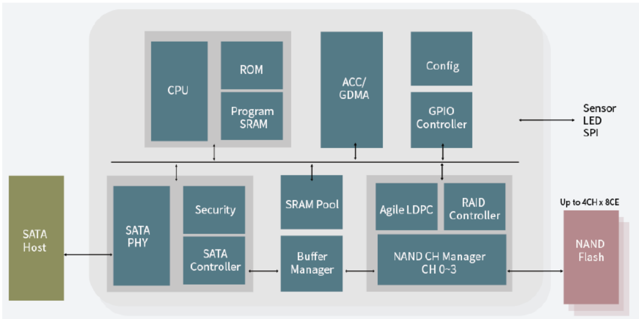
Figure 2: Innodisk 2.5" SATA SSD 3TE7 Block Diagram
