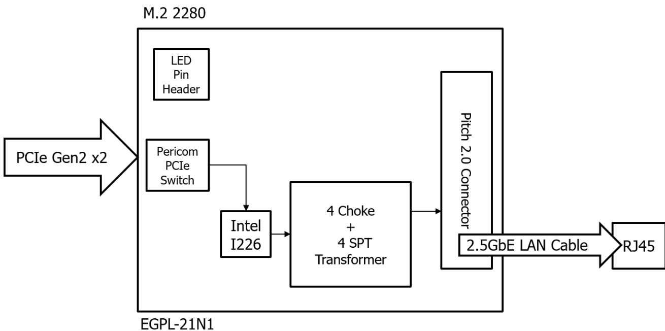
Figure 1: Block Diagram
