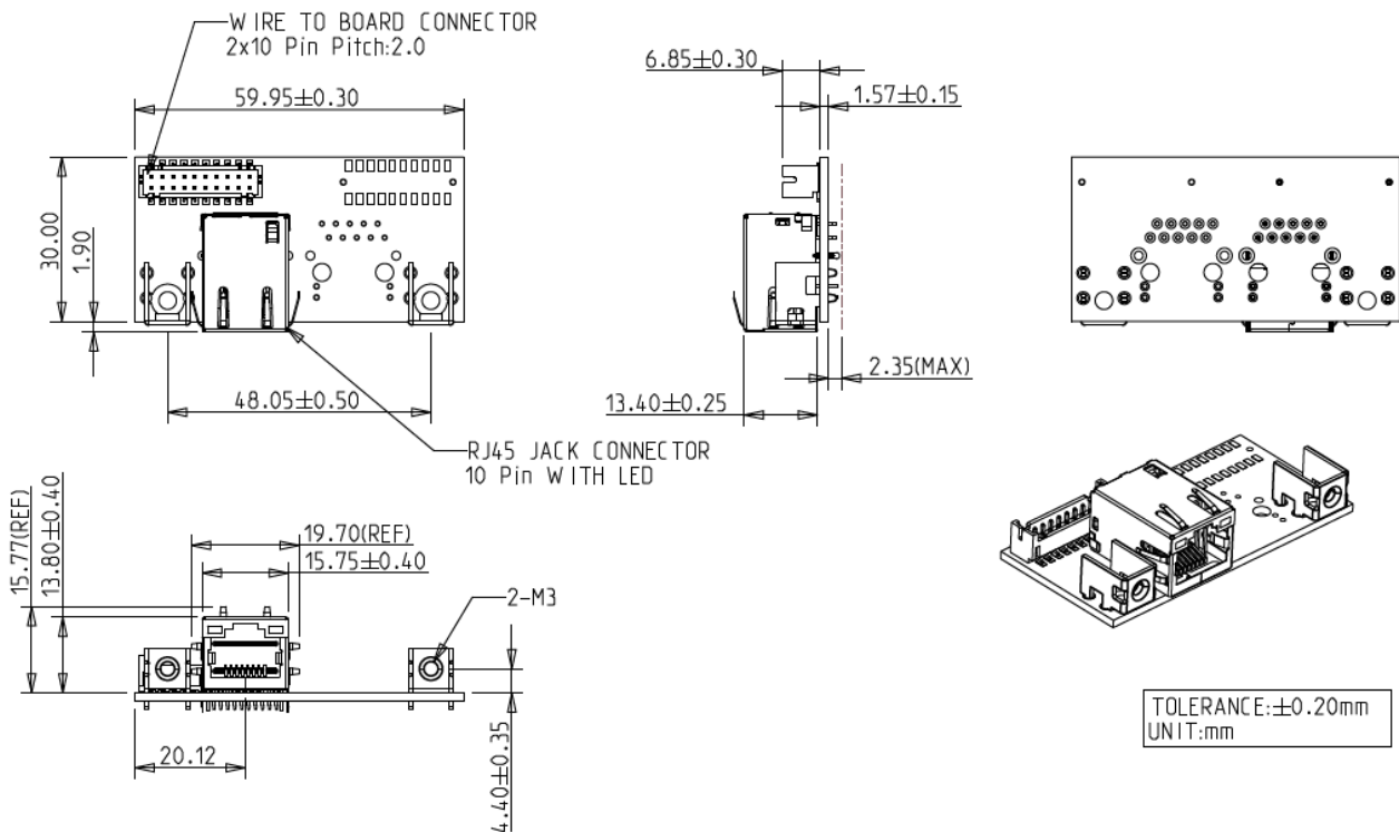
Figure 8: Mounting Hole Daughter Board Drawing (EGPL-21S1-C1/W1)
