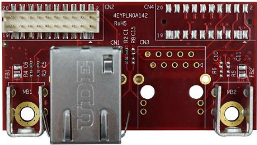
Figure 3: Mounting Hole Daughter Board Picture (EGPL-21S1-C1/W1)
