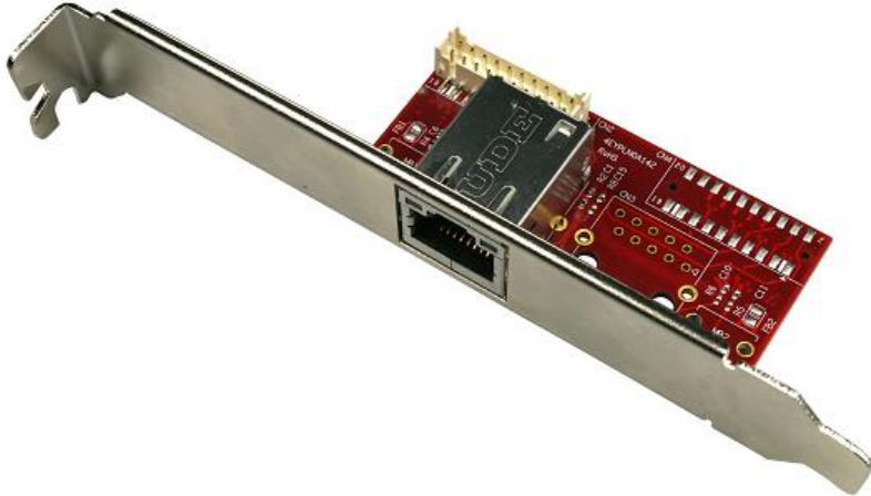
Figure 4: Bracket Daughter Board Picture (EGPL-21S1-C2/W2)
