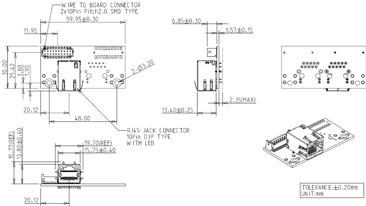
Figure 9: Bracket Daughter Board Drawing (EGPL-21S1-C2/W2)
