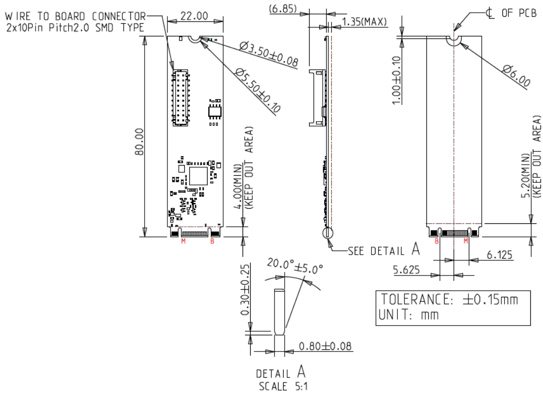
Figure 7: EGPL-21S1 M.2 Board Drawing
