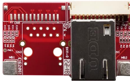
Figure 3: Mounting Hole Daughter Board Picture (EGPL-21S4-C1/W1)
