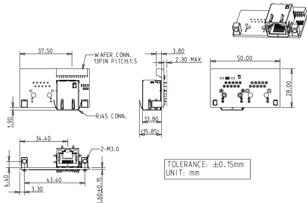
Figure 7: Mounting Hole Daughter Board Drawing (EGPL-21S4-C1/W1)
