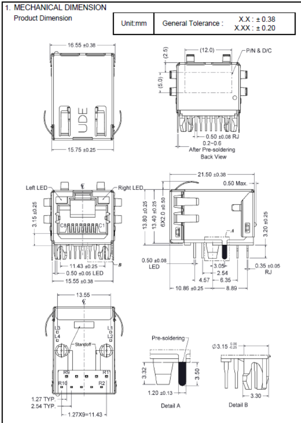
Figure 5: RJ45 Connector Drawing
