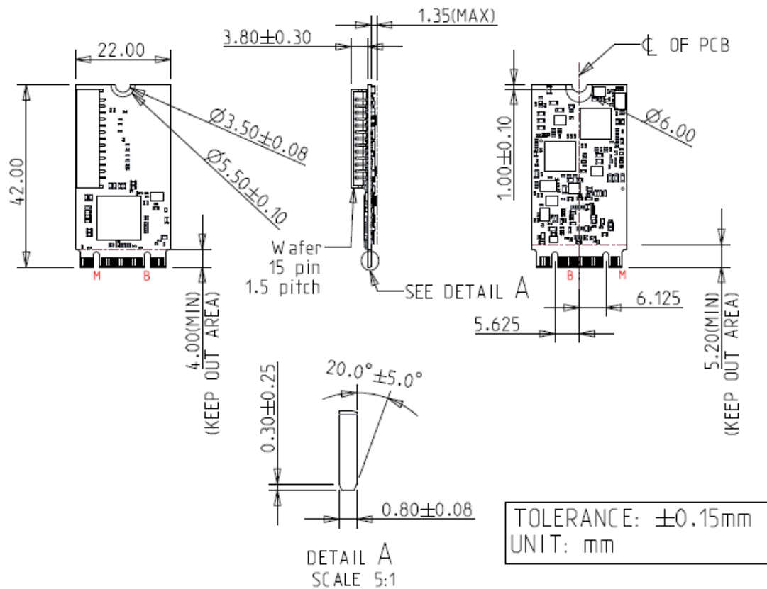
Figure 6: EGPL-21S4 M.2 Board Drawing
