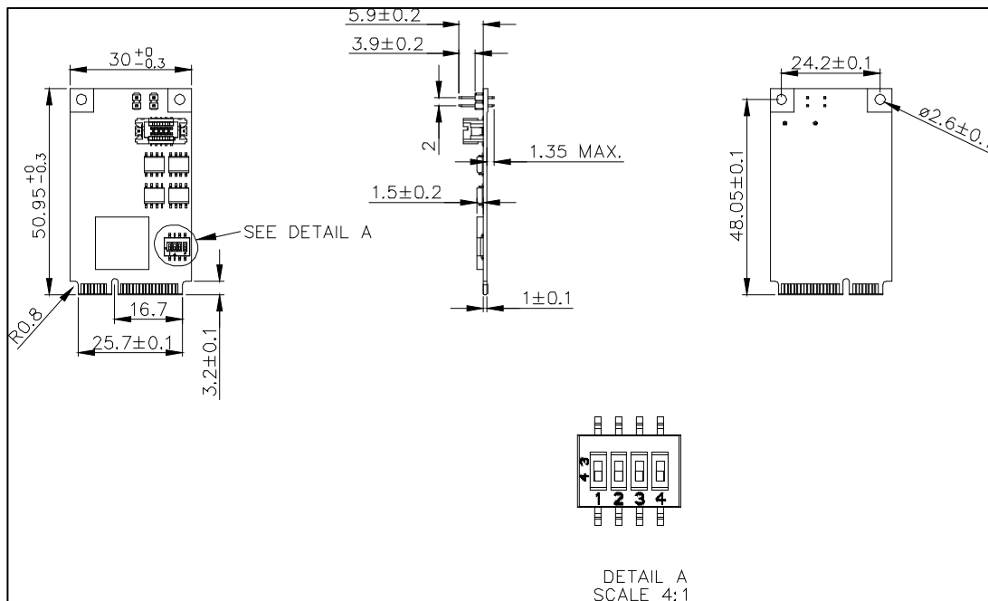
Figure 6: EMP2-X202 Drawing
