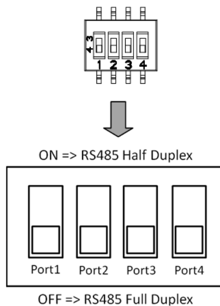
Figure 5: DIP Switch 8pin Drawing (SW1)
