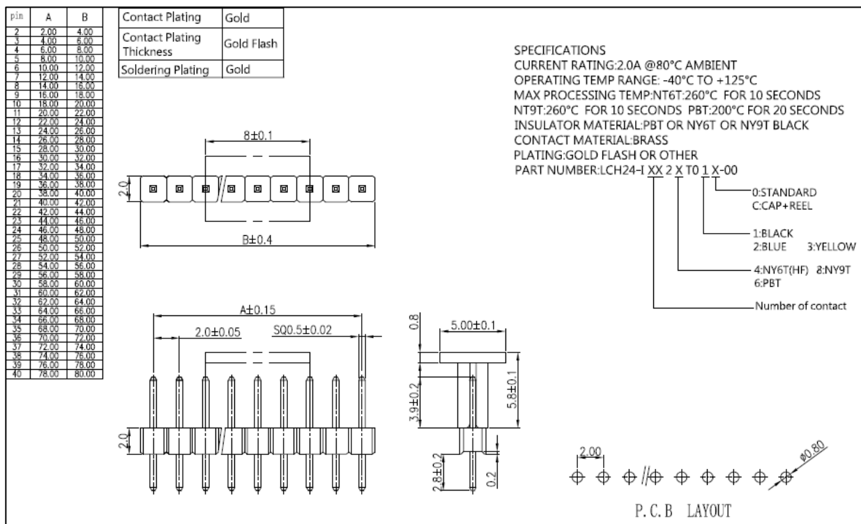
Figure 4: Pin Header DIP 1*2P Drawing (CN3/CN4)
