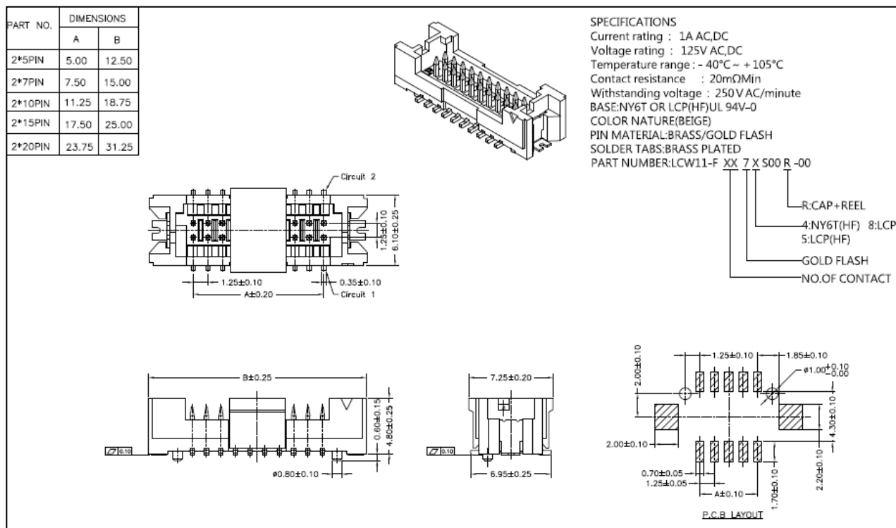
Figure 3: Wire to Board SMD 2*5P Connector Drawing (CN1)
