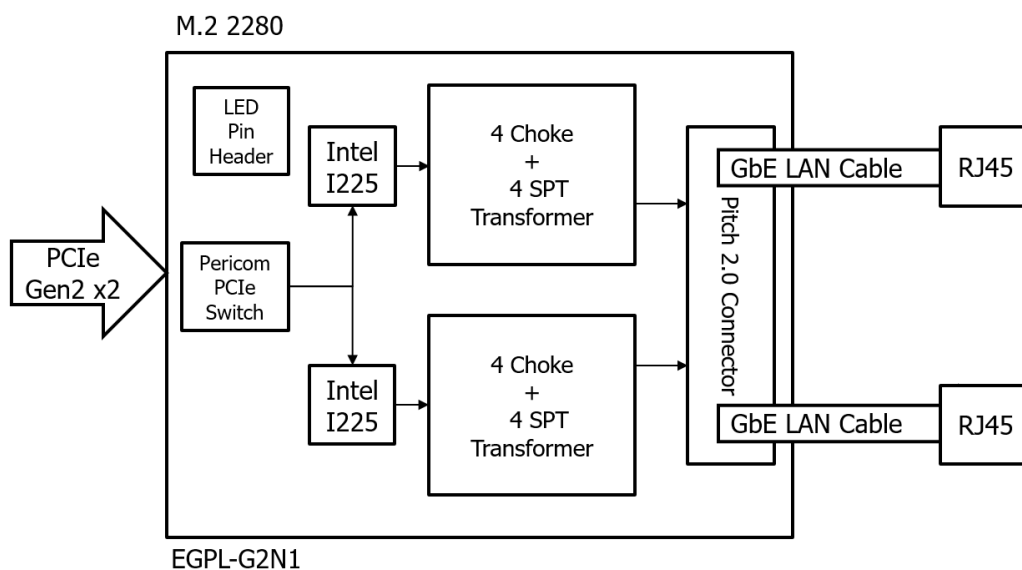
Figure 1: Block Diagram
