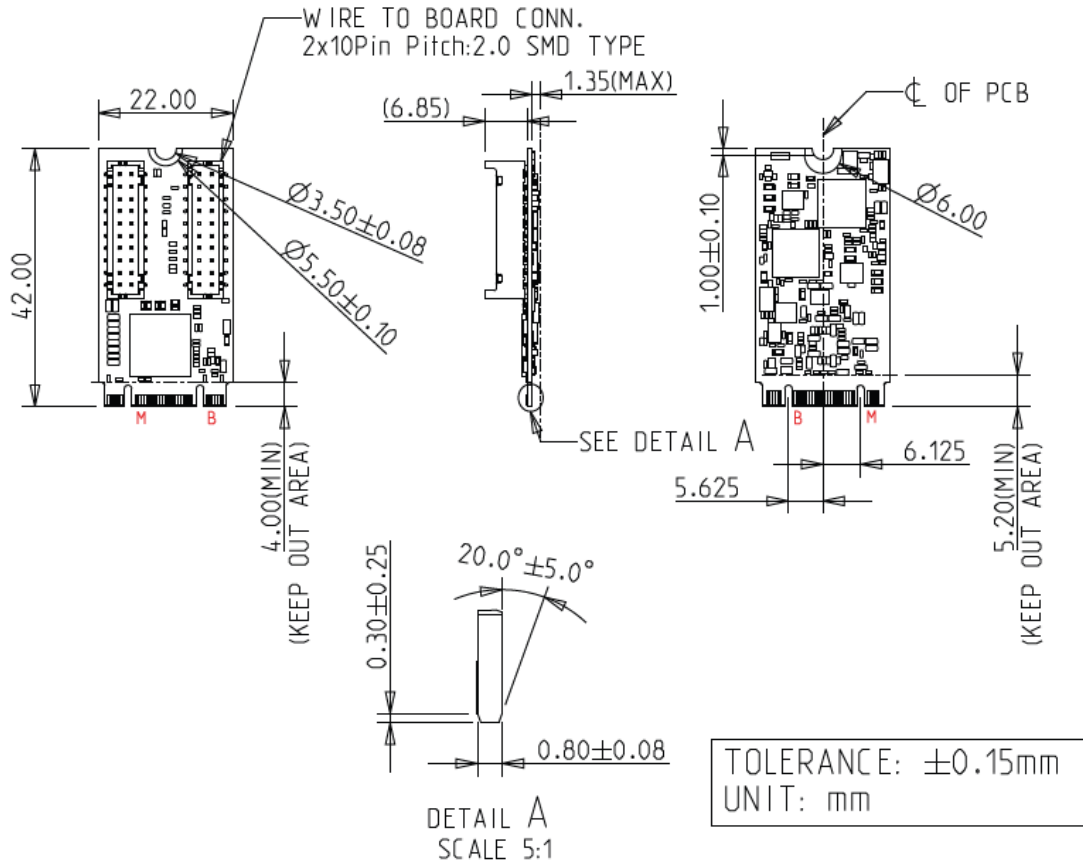
Figure 6: EGPL-G2S2 M.2 Board Drawing
