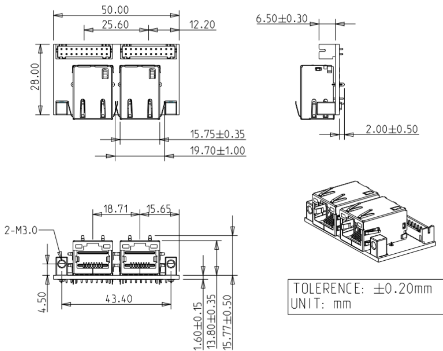
Figure 7: Mounting Hole Daughter Board Drawing
