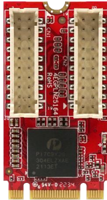
Figure 2: M.2 2242 Board Picture
