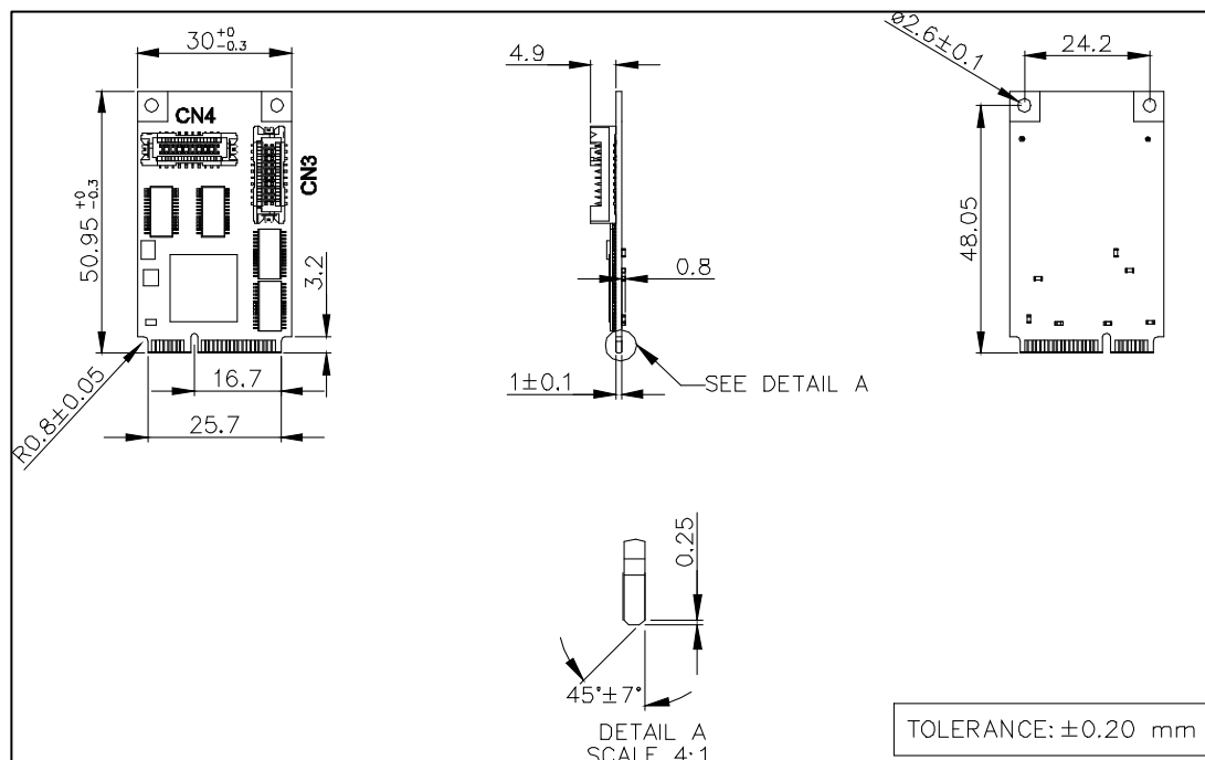
Figure 4: EMP2-X403 Drawing
