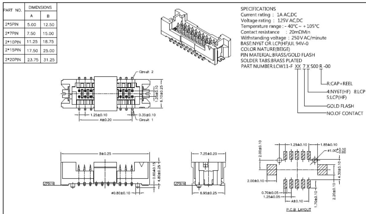
Figure 3: Wire to Board SMD 2*10P Connector Drawing (CN3/CN4)
