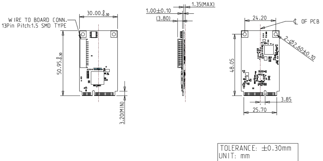
Figure 7: EMPL-G1S2 mPCIe Board Drawing
