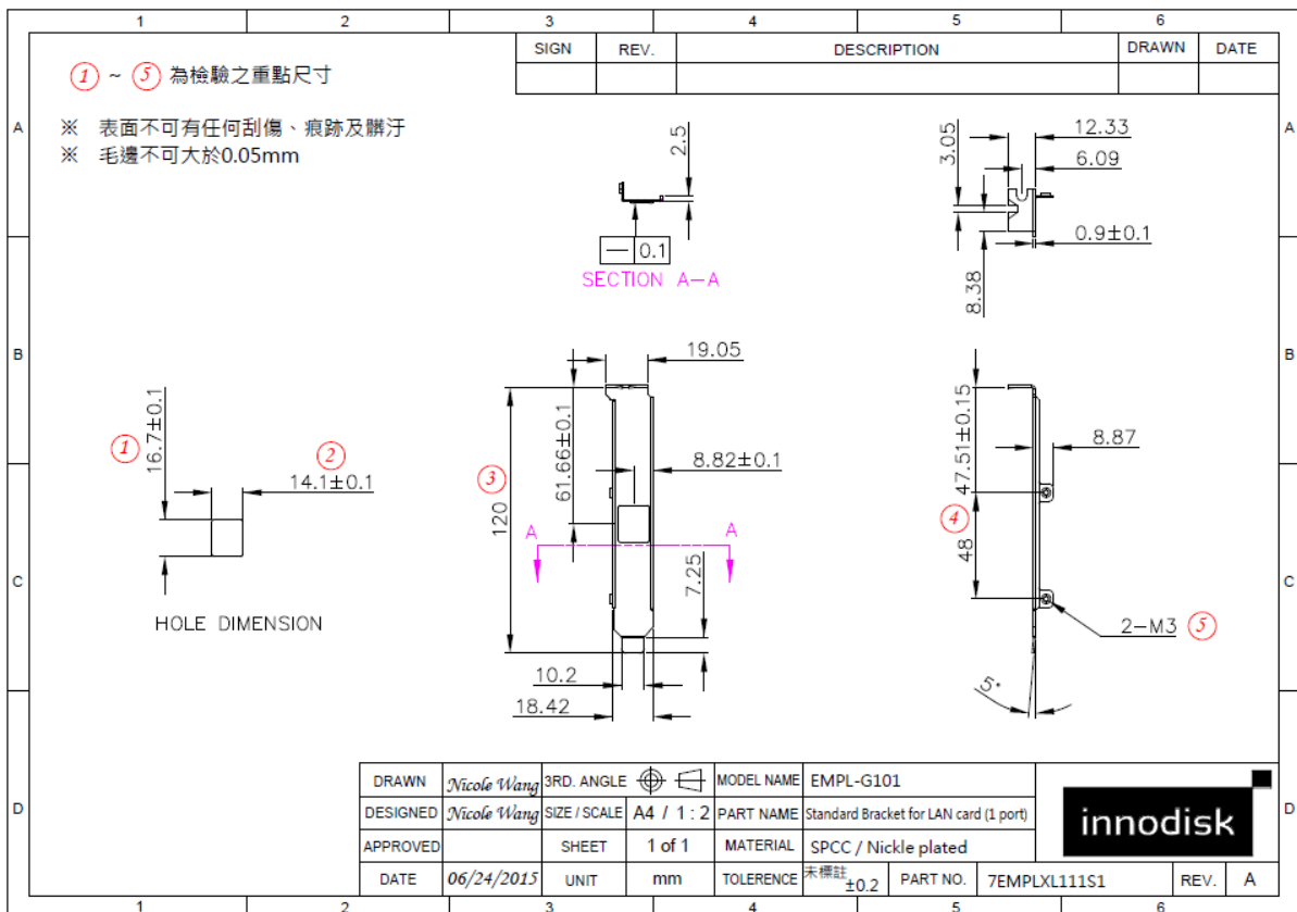
Figure 10: Bracket Drawing
