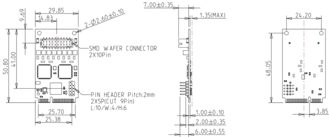
Figure 5: EMPL-G203 mPCIe Board Drawing
