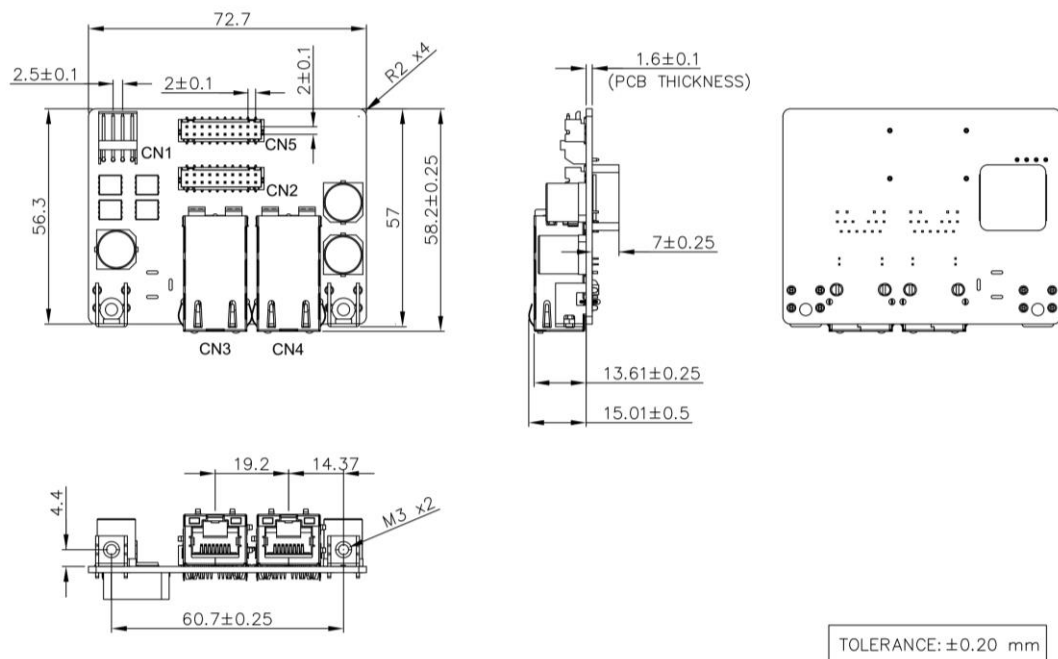
Figure 10: Mounting Hole Daughter Board Drawing - 4Pin Header (EMPL-G2P1-C1/W1)
