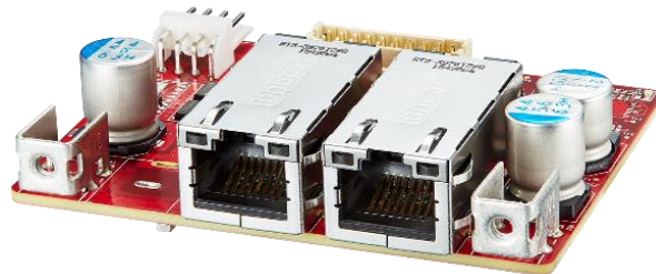
Figure 3: Mounting Hole, 4Pin Header, Daughter Board Picture (EMPL-G2P1-C1/W1)
