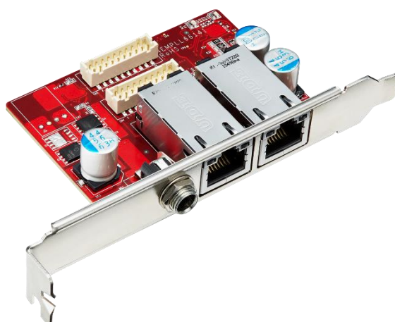
Figure 6: Bracket, DC Jack, Daughter Board Picture (EMPL-G2P1-C4/W4)
