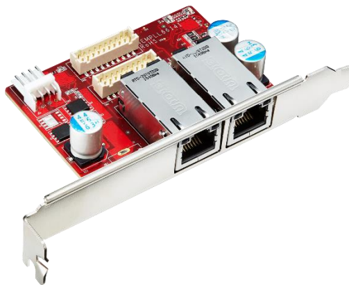
Figure 4: Bracket, 4Pin Header, Daughter Board Picture (EMPL-G2P1-C2/W2)
