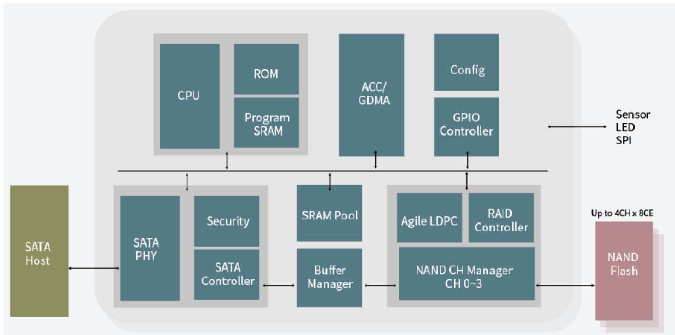
Figure 3: Innodisk M.2 (S80) 3IE7 Block Diagram
