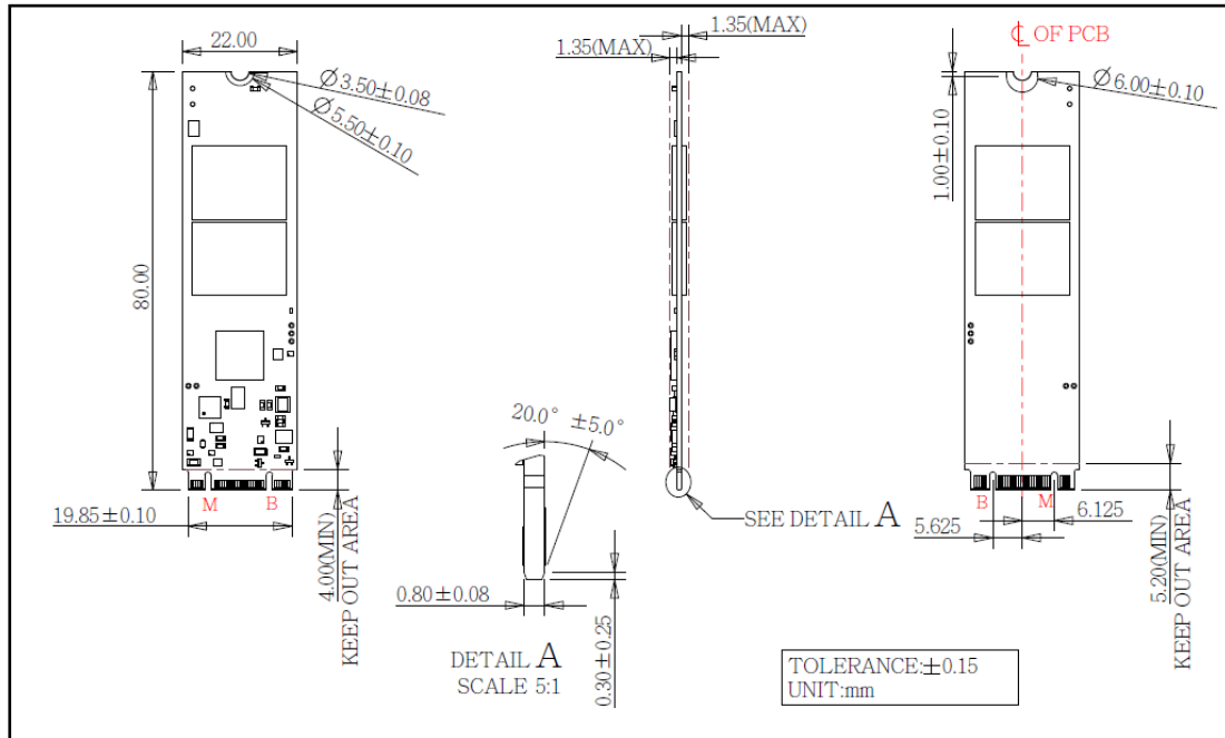
Figure 2: Innodisk M.2 (S80) 3IE7 diagram (BGA)
