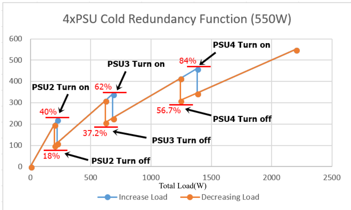
Figure 9 –4xPSU Cold Redundancy Function (550W)
