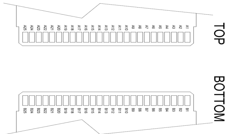
Figure 10 – Card Edge Dimension
