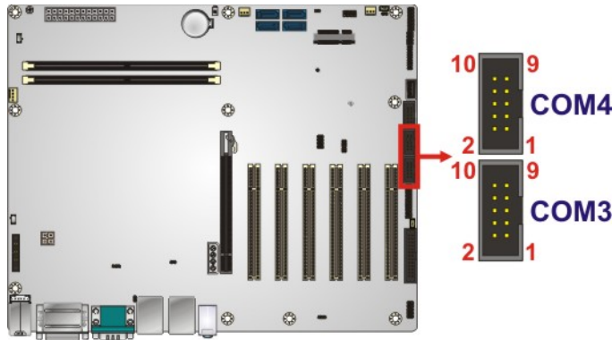
Figure 3-24: RS-232 Serial Port Connector Locations
