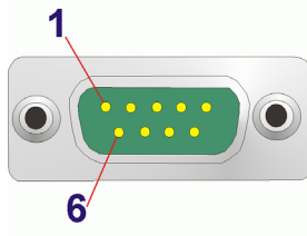
Figure 3-37: Serial Port Connector Pinouts
