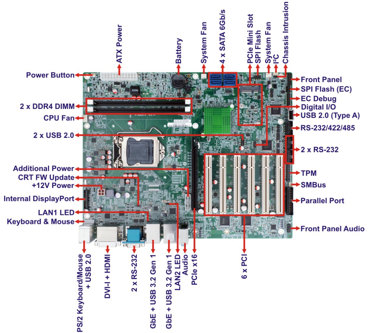
Figure 1-2: Connectors
