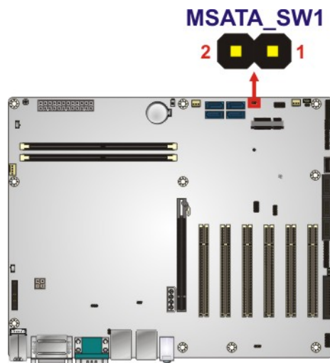
Figure 4-17: mSATA Setup Jumper Location
