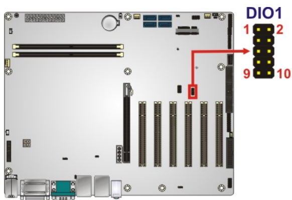
Figure 3-9: Digital I/O Connector Location
