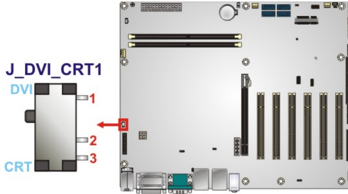
Figure 4-15: DVI/CRT Selection Switch Location
