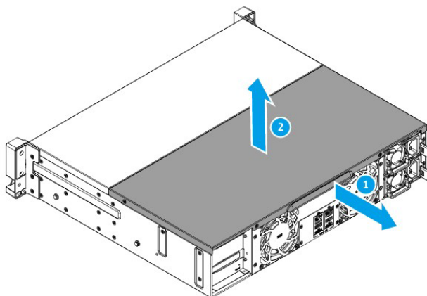
Figure 3-2: Remove the Case Cover
