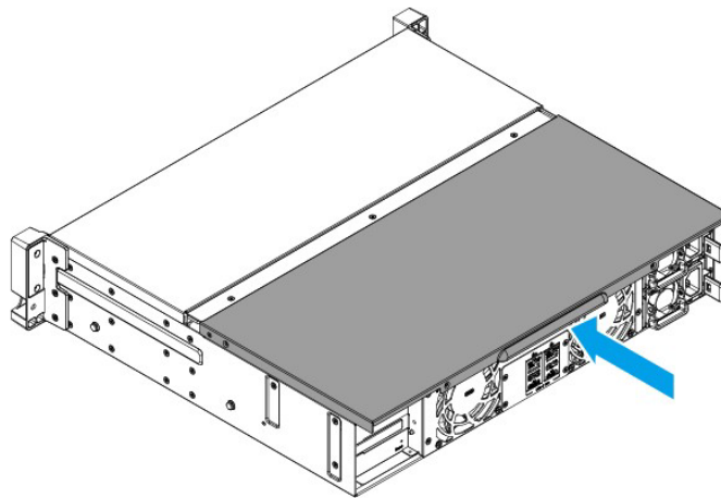
Figure 3-4: Slide the Cover
