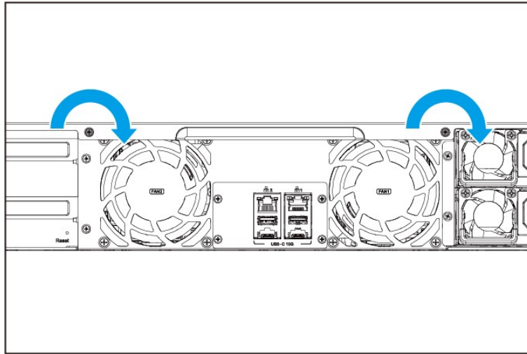
Figure 3-5: Tighten Captive Screws
