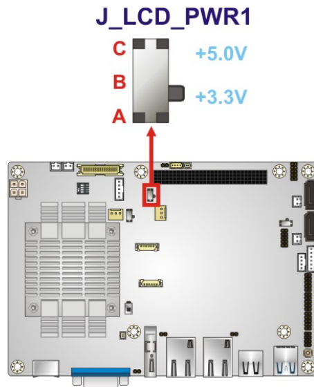
Figure 4-7: LCD Voltage Selection Switch Location
