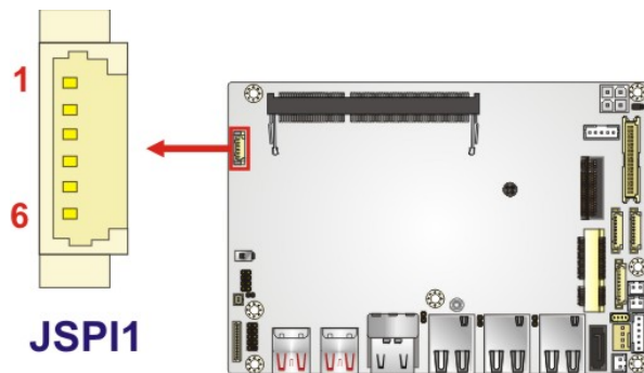
Figure 3-21: SPI Flash Connector Location
