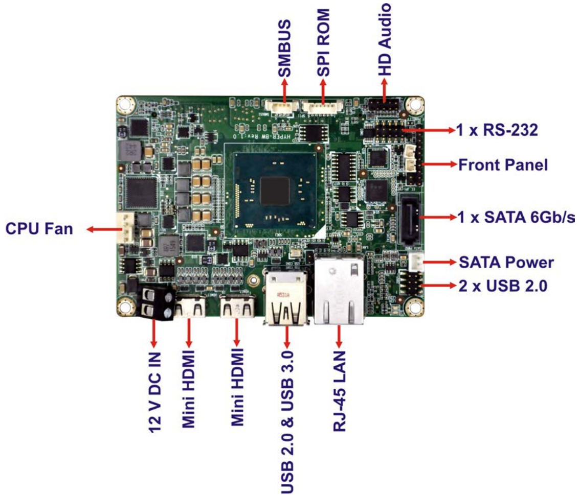
Figure 1-2: Connectors (Front Side)
