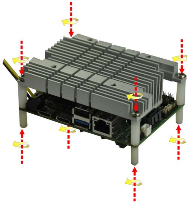
Figure 4-7: Heat Sink Retention Screws
