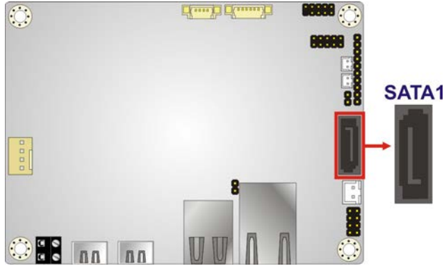
Figure 3-17: SATA 6Gb/s Drive Connector Location
