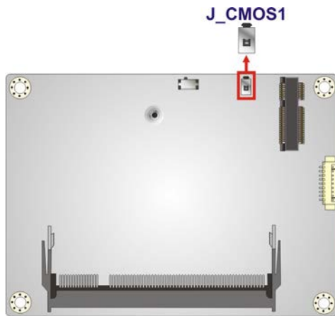
Figure 3-8: Clear CMOS Button Location
