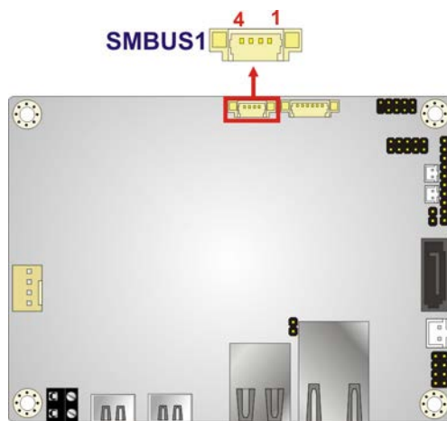
Figure 3-19: SMBus Connector Location
