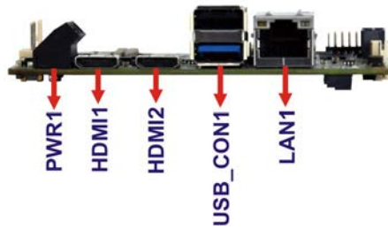
Figure 3-21: External Peripheral Interface Connector
