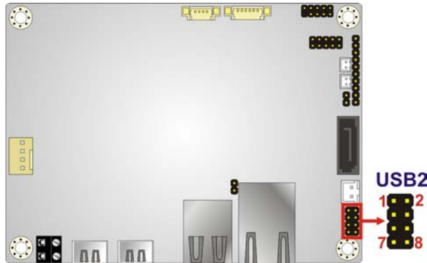
Figure 3-20: USB Connector Location
