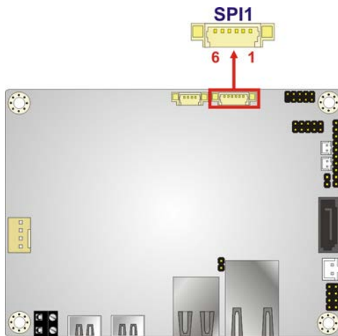
Figure 3-6: BIOS FW Connector Location
