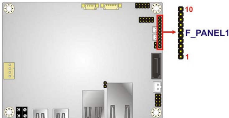
Figure 3-13: Front Panel Connector Location
