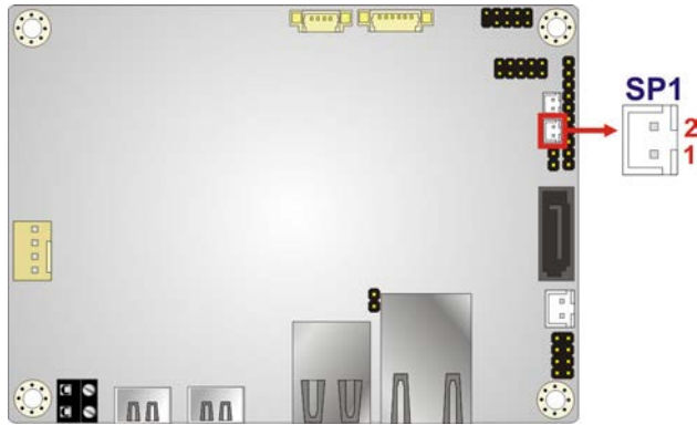
Figure 3-7: Buzzer Connector Location
