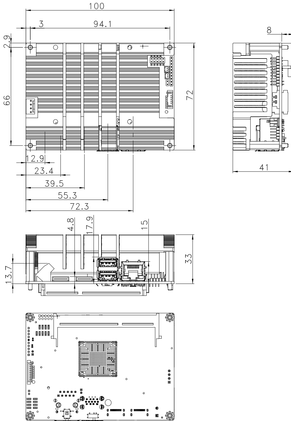
Figure 1-4: Dimensions (mm)
