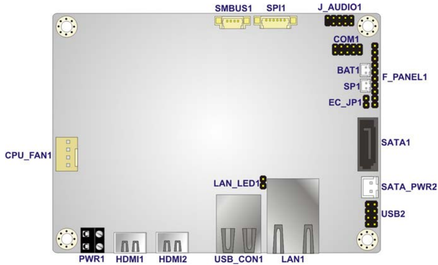
Figure 3-1: Connector and Jumper Locations (Front)
