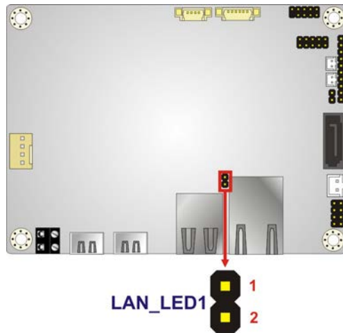
Figure 3-14: LAN LED Connector Locations
