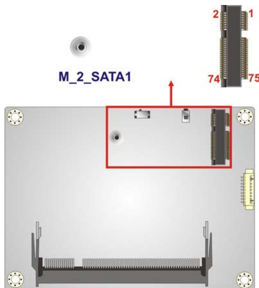
Figure 3-15: M.2 2242 (B key) Slot Location
