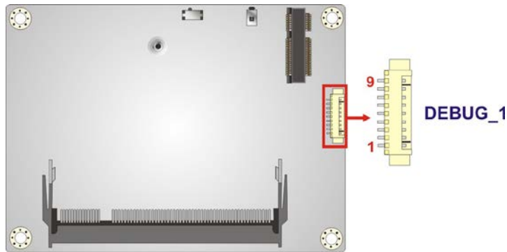
Figure 3-11: Debug Port Connector Location
