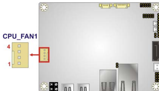
Figure 3-9: CPU Fan Connector Location
