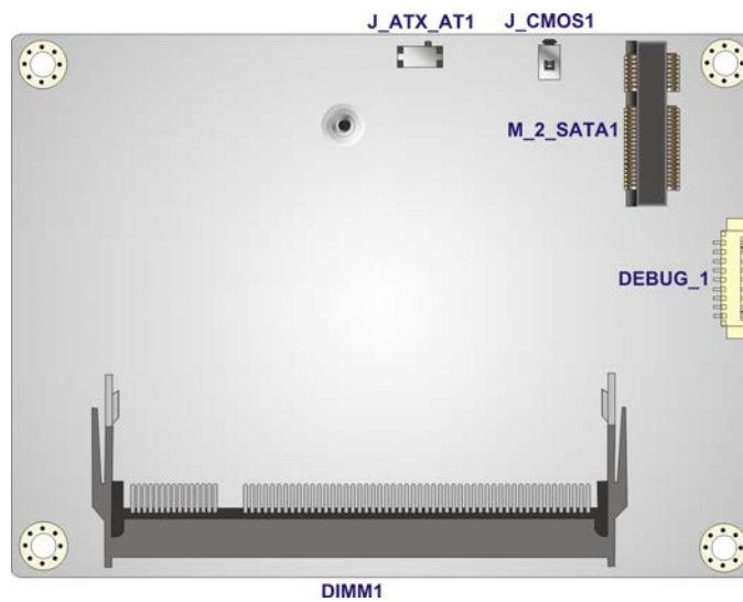
Figure 3-2: Connector and Jumper Locations (Rear)
