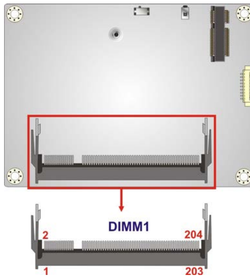
Figure 3-10: DDR3L SO-DIMM Slot Location
