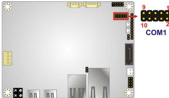
Figure 3-16: RS-232 Serial Port Connector Location
