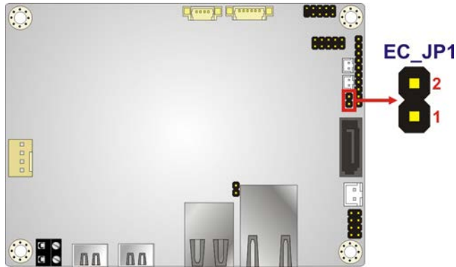
Figure 3-12: EC FW Connector Location
